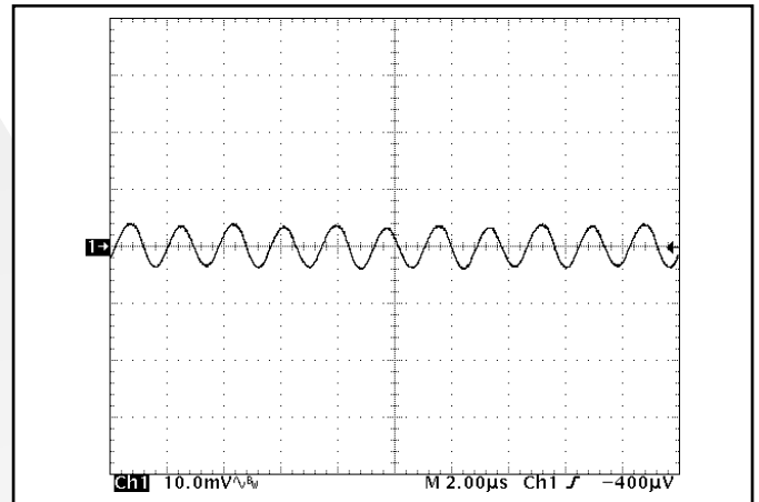
Figure 16: Output voltage ripple, V_{out} , at nominal input voltage and rated load current (10 mV/div). Load capacitance: 1µF ceramic capacitor and 10µF tantalum capacitor. Bandwidth: 10 MHz. See Figure 14.
