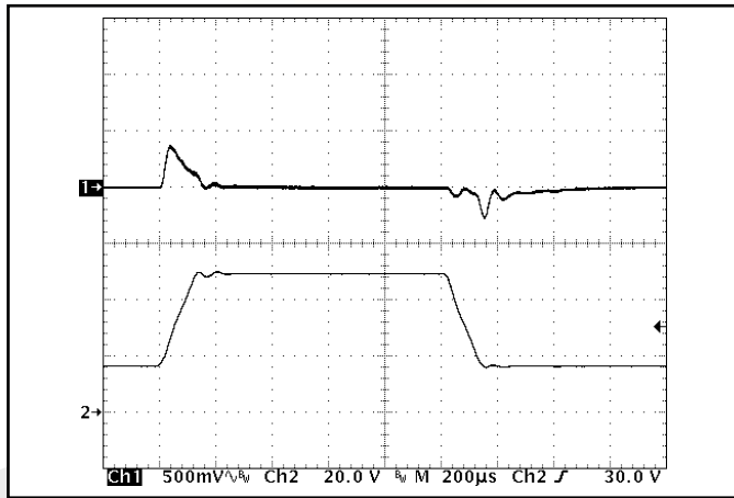
Figure 13: Output voltage response to step-change in input voltage (16V - 50V - 16V). Load cap: 10µF, 100 mΩ ESR tantalum cap and 1µF ceramic cap. Ch 1: Vout (500mV/div). Ch 2: Vin (20V/div).
