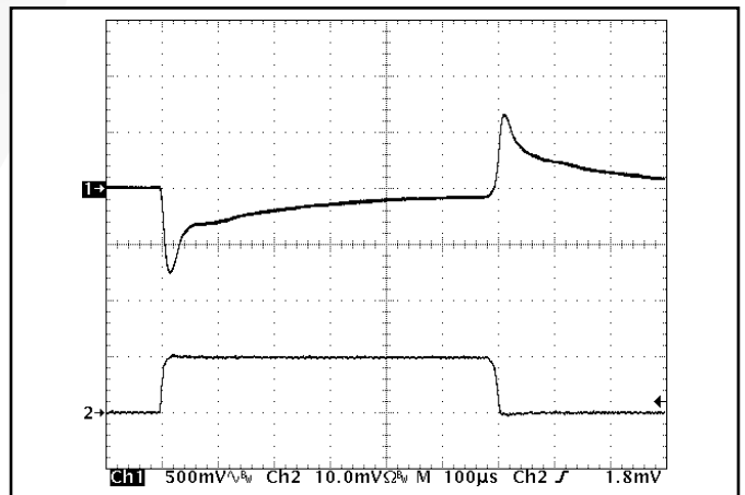
Figure 12: Output voltage response to step-change in load current (0%-50%-0% of Iout(max)). Load cap: 1µF ceramic cap and 10µF, 100 mΩ ESR tantalum cap. Ch 1: Vout (500mV/div). Ch 2: Iout (2A/div).
