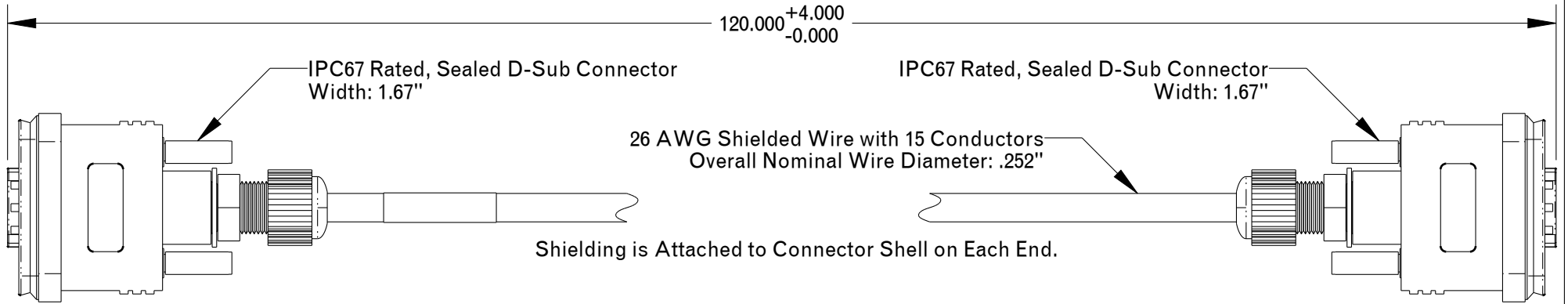
DB15 Male
