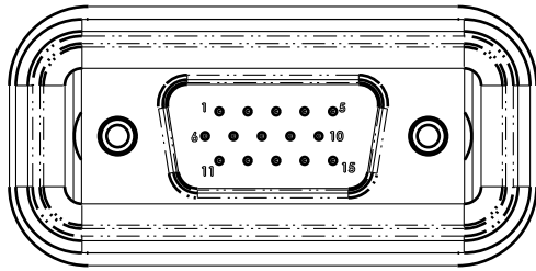
DB15 Male
