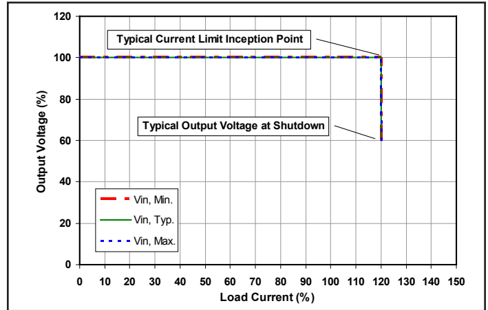
Common Figure 2: Output voltage vs. load current showing typical current limit inception points and converter shutdown points.
