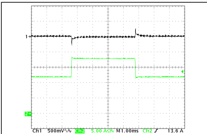
Figure 5: Output voltage response to step-change in load current (50%-75%-50% of Iout(max); dI/dt = 0.1A/us). Load cap: 15µF tantalum cap and 1µF ceramic cap. Ch 1: Vout, Ch 2: Iout.
