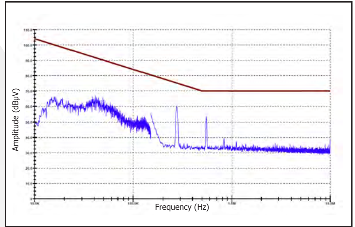
Figure 4: MIL-STD-461E Method CE102 High Frequency Conducted Emissions. Limit line (in brown) is the 'Basic Curve'. Setup described on page 6.
