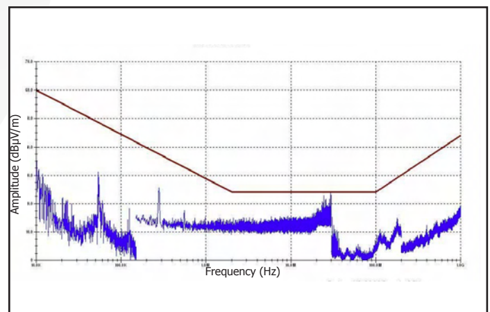
Figure 6: MIL-STD-461E Method RE102 High Frequency Radiated Emissions. Limit line (in brown) is the 'Submarine External to Pressure Hull Curve'. Setup described on page 6.
