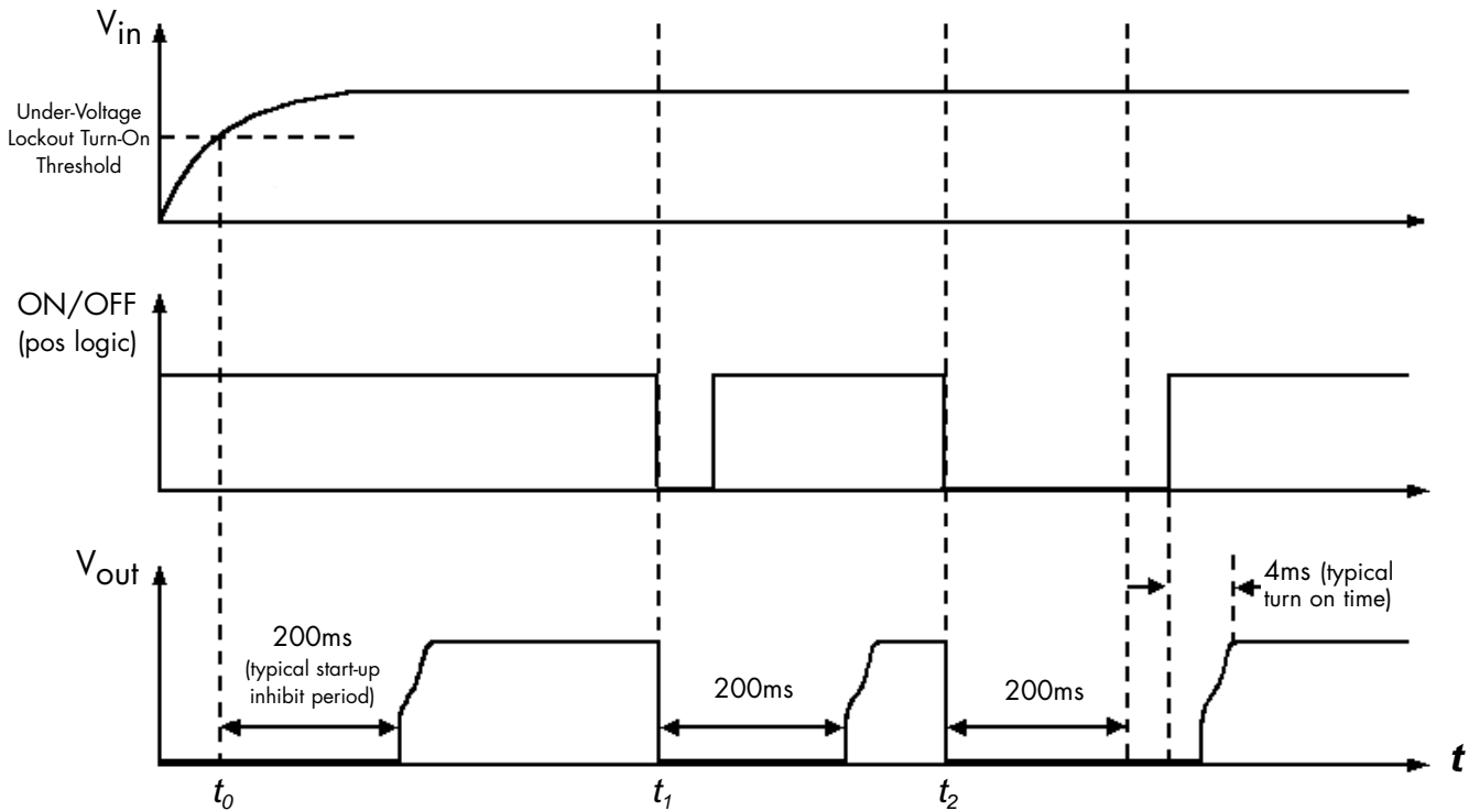
Figure 1: Standard Startup Inhibit Period - "S" option (turn-on & inhibit time not to scale)
