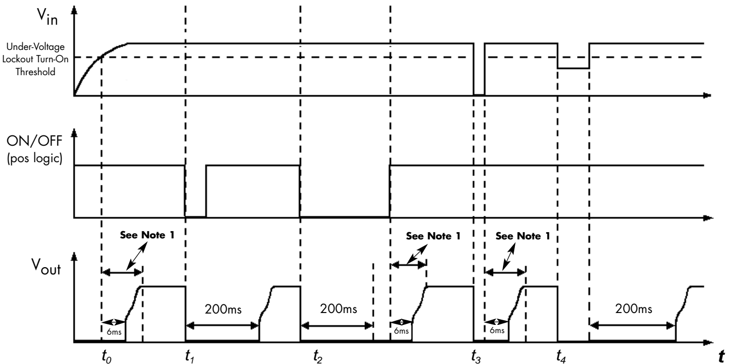
Figure 2: Alternative Startup Inhibit Period - "Y" option (turn-on & inhibit time not to scale)
