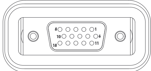
DB15 Female
