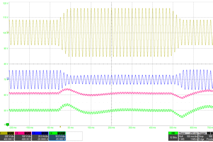
Figure 7: Input transient with 600µF hold-up capacitor at full load (115Vrms-220Vrms-115Vrms, 60Hz) Ch1: Vin (200V/div), Ch2: Vhold-up (100V/div), Ch3: Iin (20A/div), Ch4: Vout (10V/div), Timebase: (100ms/div).
