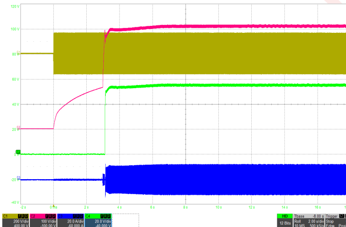
Figure 3: Typical startup waveform with 600µF hold-up capacitor (115Vrms, 60Hz) Ch1: V_{in} (200V/div), Ch2: Hold-up capacitor voltage (100V/div), Ch3: I_{in} (20A/div), Ch4: V_{out} (20V/div), Timebase: (2s/div).
