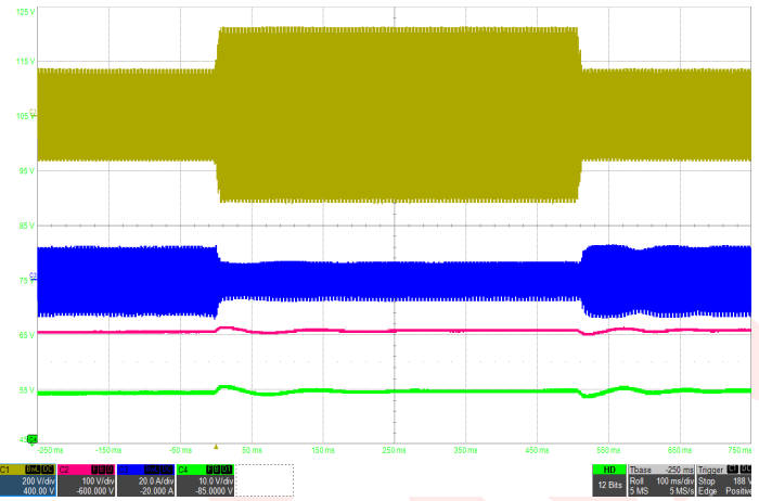
Figure 8: Input transient with 600µF hold-up capacitor at full load (115Vrms-220Vrms-115Vrms, 400Hz) Ch1: Vin (200V/div), Ch2: Vhold-up (100V/div), Ch3: Iin (20A/div), Ch4: Vout (10V/div), Timebase: (100ms/div).
