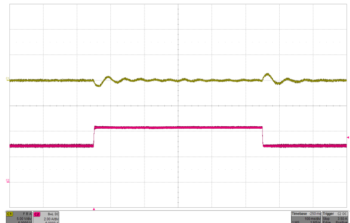
Figure 12: Regulated model output voltage response to step-change in load current with 200µF hold-up capacitor (50%-75%-50% of Iout(max), 115Vrms, 400Hz) Top: Vout (5V/div), Bottom: Iout (2A/div), Timebase: (100ms/div).
