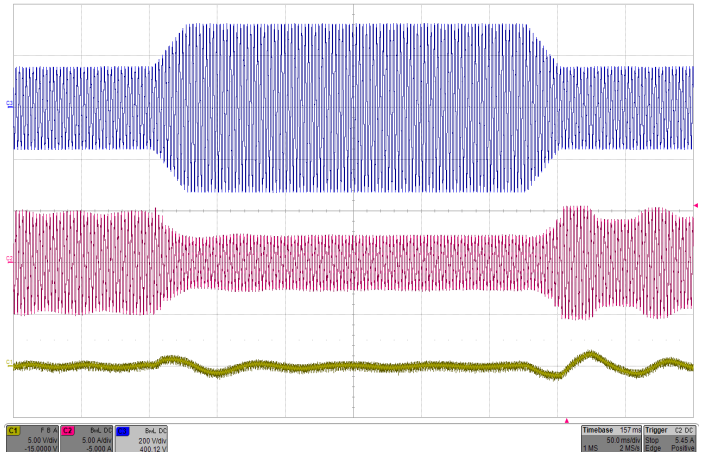
Figure 16: Input voltage transient response with 200µF hold-up capacitor at full load current (115Vrms-230Vrms-115Vrms, 400Hz), Top: Vin (200V/div), Mid: Iin (5A/div), Bottom: Vout (5V/div), Timebase: (50ms/div).
