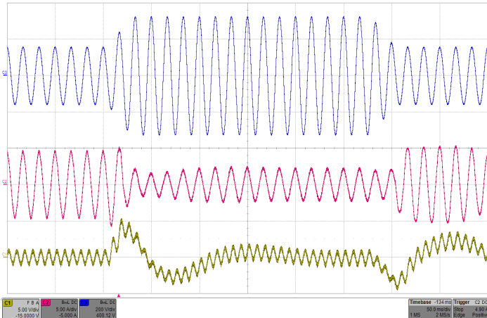
Figure 15: Input voltage transient response with 200µF hold-up capacitor at full load current (115Vrms-230Vrms-115Vrms, 60Hz), Top: Vin (200V/div), Mid: Iin (5A/div), Bottom: Vout (5V/div), Timebase: (50ms/div).
