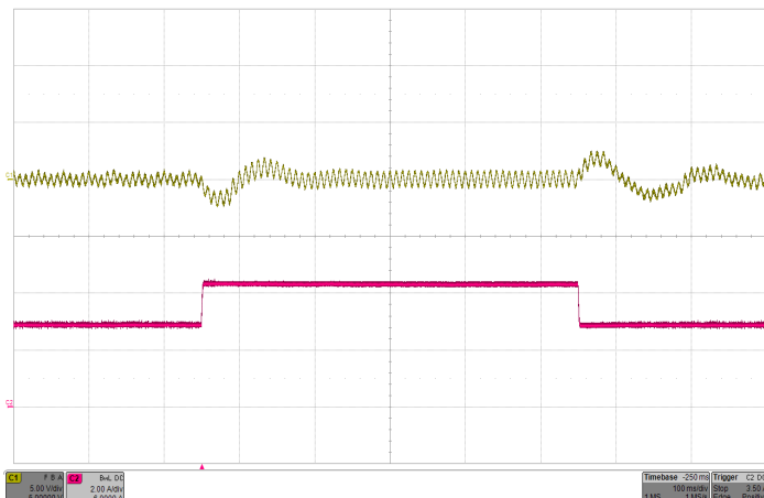
Figure 11: Regulated model output voltage response to step-change in load current with 200µF hold-up capacitor (50%-75%-50% of Iout(max), 115Vrms, 60Hz) Top: Vout (5V/div), Bottom: Iout (2A/div), Timebase: (100ms/div).
