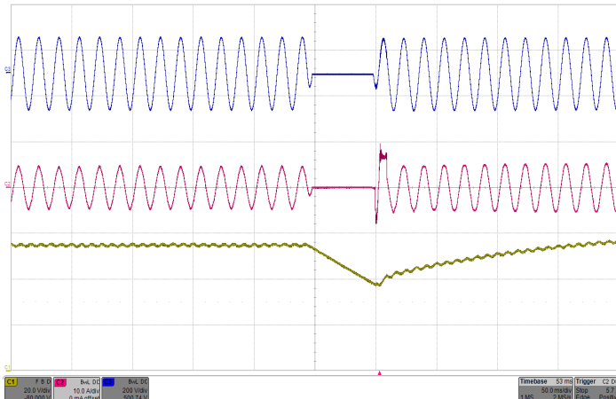
Figure 9: Line drop out with 400µF hold-up capacitor at full load current (115Vrms, 60Hz) Top: Vin (200V/div), Mid: Iin (10A/div), Bottom: Vout (20V/div), Timebase: (50ms/div).
