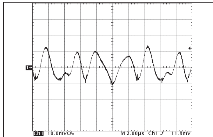
Figure 14: Input reflected ripple current, i_s , through a 10\ \mu\text{H} source inductor at nominal input voltage and rated load current (20 mA/div). See Figure 12.
