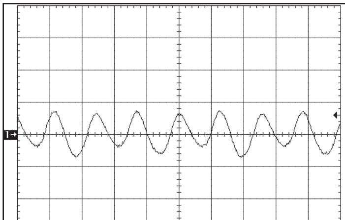
Figure 13: Input Terminal Ripple Current, i_c , at full rated output current and nominal input voltage with 10\ \mu\text{H} source impedance and 47\ \mu\text{F} electrolytic capacitor (500 mA/div). See Figure 12.
