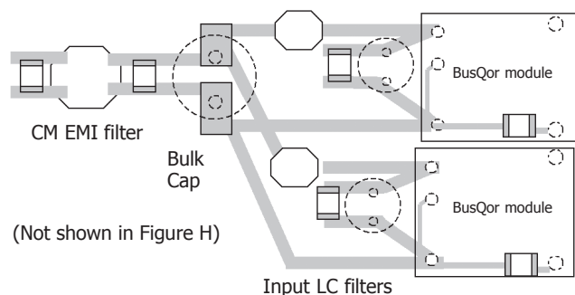
Figure J: Recommended PCB layout for input circuit
