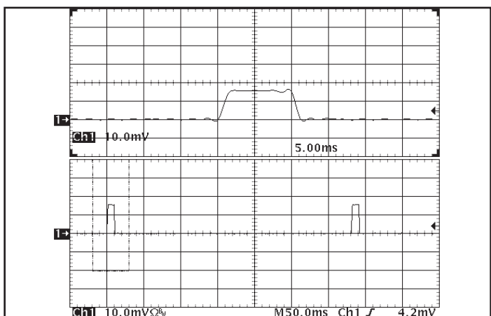
Figure 17: Load current (50 A/div) as a function of time when the converter attempts to turn on into a 1\ \text{m}\Omega short circuit. Top trace (5.0 ms/div) is an expansion of the on-time portion of the bottom trace.
