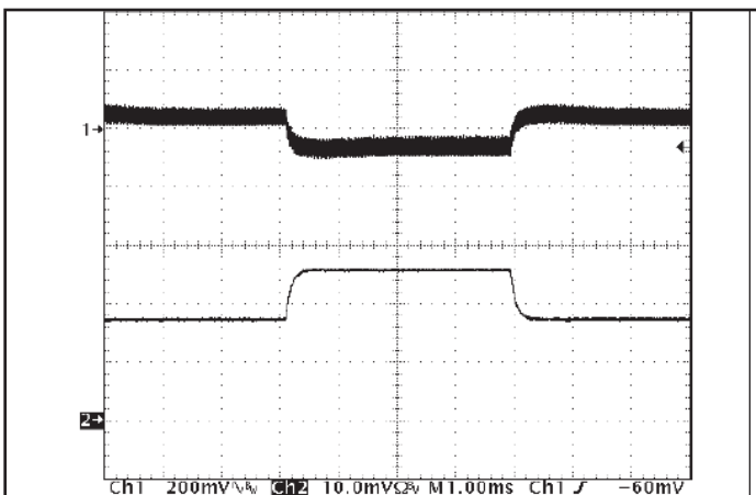
Figure 11: Output voltage response to step-change in load current (50%-75%-50% of I_{out(max)} ; dI/dt = 0.1 \text{ A}/\mu\text{s} ). Load cap: 15 \mu\text{F} tantalum cap and 1 \mu\text{F} ceramic cap. Top trace: V_{out} (200 mV/div), Bottom trace: I_{out} (5 A/div).
