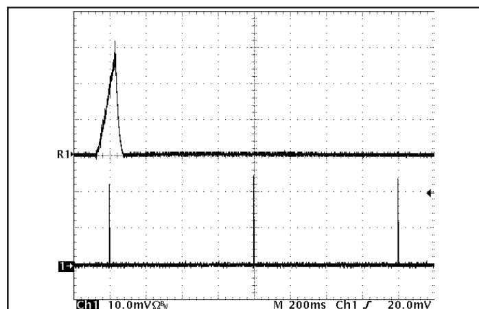
Figure 18: Load current (50 A/div) as a function of time when the converter attempts to turn on into a 1 m \Omega short circuit. Top trace (1 ms/div) is an expansion of the on-time portion of the bottom trace.
