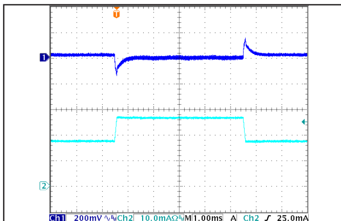
Figure 5: Output voltage response to step-change in load current (66 % -100 % -66 % of I out (max); dI/dt = 0.1 A/μs). Load cap: 1 μF ceramic capacitor. Ch 1: V out (200 mV/div), Ch 2: I out (10 A/div).
