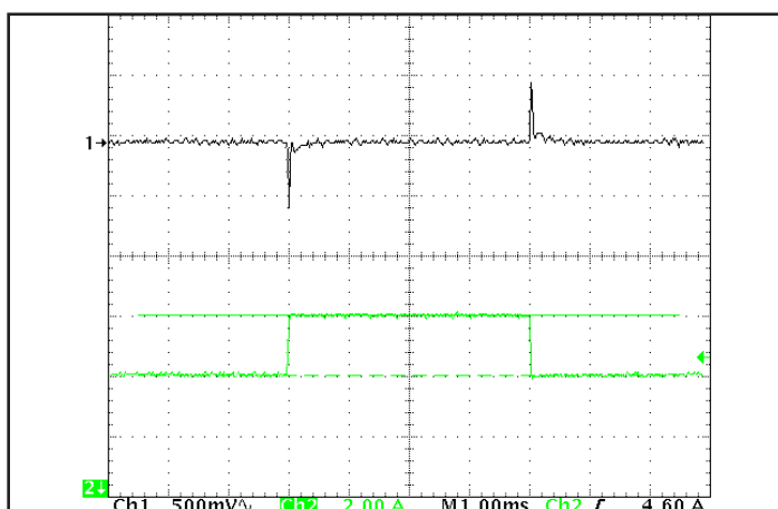
Figure 5: Output voltage response to step-change in load current (50% - 75% - 50% of Iout(max); dI/dt = 0.1 A/μs). Load cap: 15 μF tantalum cap and 1 μF ceramic cap. Ch 1: Vout (500 mV/div), Ch 2: Iout (2 A/div). Timebase: (1 ms/div).
