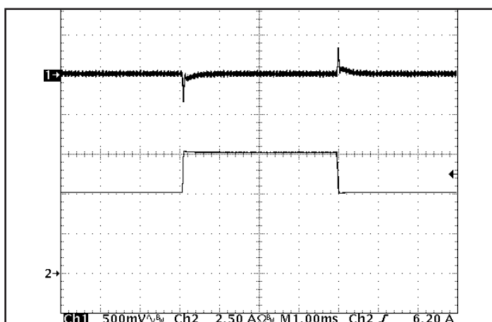
Figure 5: Output voltage response to step-change in load current (50%-75% -50% of I out (max); dI/dt = 0.1 A/μs). Load cap: 15 μF tantalum cap and 1 μF ceramic cap. Ch 1: V out , (500 mV/div), Ch 2: I out (2.5 A/div). Timebase: (1 ms/div).
