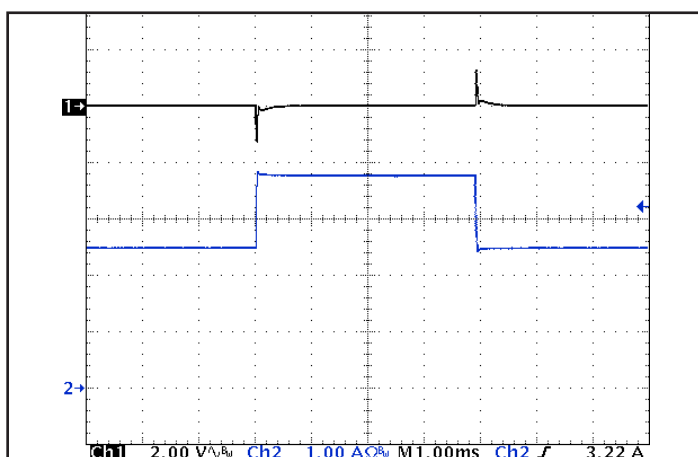
Figure 5: Output voltage response to step-change in load current (50%-75% -50% of I out (max); dI/dt = 0.8 A/μs). Load cap: 1 μF ceramic cap. Ch 1: V out , (2 V/div), Ch 2: I out (1 A/div). Timebase: (1 ms/div).
