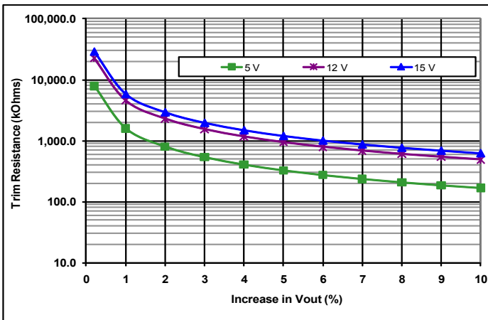
Common Figure 3: Trim graph for trim-up 5.0 to 15 V outputs.
