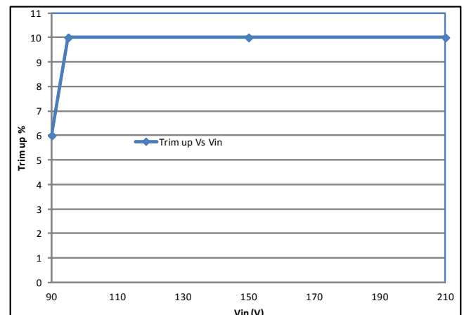
Common Figure 6: Trim up vs. Input voltage.
