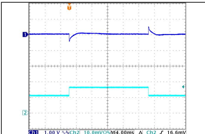
Figure 5: Output Voltage Response to Step-Change in Load Current (50% -75% -50% of Iout(max); dI/dt = 0.1 A/μs). Load cap: 15 μF tantalum cap and 1 μF ceramic cap. Ch 1: Vout (1.00 V/div), Ch 2: Iout (10.0 A/div). Timescale: 4.00 ms/div.
