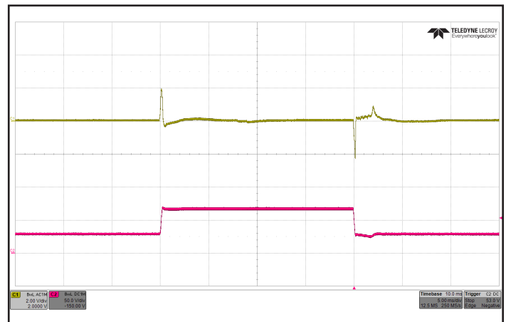
Figure 6: Output Voltage Response to Step-Change in Input Voltage (250 V/ms), at Max. load current. Load cap: 330 μF electrolytic cap and 1 μF ceramic cap. Ch 1: Vout (2.00 V/div), Ch 2: Vin (50.0 V/div). Timescale: 5.00 ms/div.
