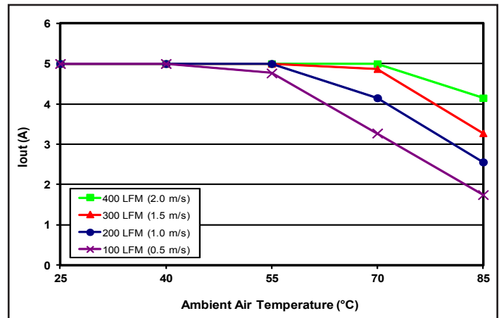
Figure 4: Thermal Derating (max output current vs. ambient air temperature) for encased converter with 1/2" heatsink, at airflow rates of 100 LFM through 400 LFM. Air flows across the converter from input to output (nominal input voltage).
