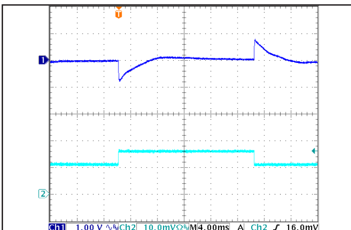
Figure 5: Output Voltage Response to Step-Change in Load Current (50% -75% -50% of Iout(max); dI/dt = 0.1 A/μs). Load cap: 100 μF electrolytic cap and 1 μF ceramic cap. Ch 1: Vout (1.00 V/div), Ch 2: Iout (5.00 A/div). Timescale: 4.00 ms/div.
