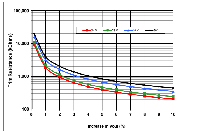
Common Figure 4: Trim-Up Graph for 24 to 50 V outputs.
