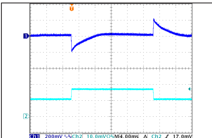
Figure 5: Output Voltage Response to Step-Change in Load Current (50% -75% -50% of I out (max); dI/dt = 0.1 A/μs). Load cap: 15 μF tantalum cap and 1 μF ceramic cap. Ch 1: V out (200 mV/div), Ch 2: I out (20.0 A/div). Timescale: 4.00 ms/div.
