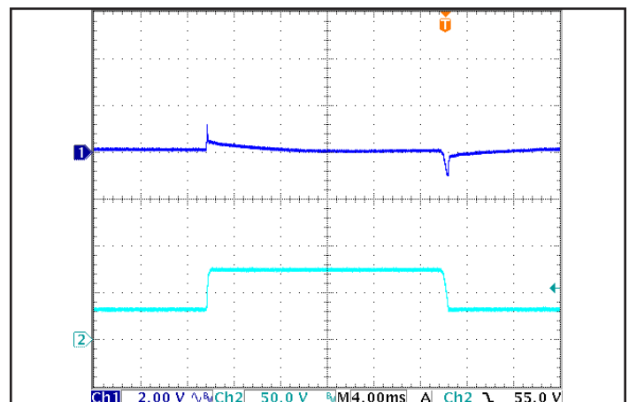
Figure 6: Output Voltage Response to Step-Change in Input Voltage (250 V/ms), at Max. load current. Load cap: 330 μF electrolytic cap and 1 μF ceramic cap. Ch 1: V out (2.00 V/div), Ch 2: V in (50.0 V/div). Timescale: 4.00 ms/div.
