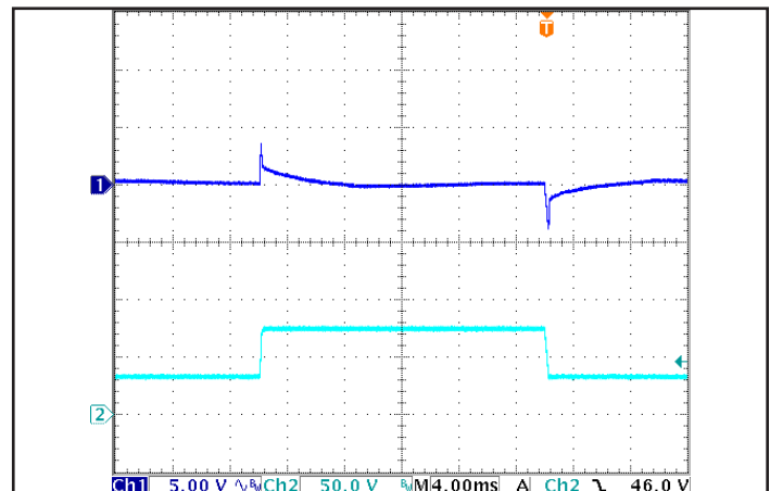
Figure 6: Output Voltage Response to Step-Change in Input Voltage (250 V/ms), at Max. load current. Load cap: 330 μF electrolytic cap and 1 μF ceramic cap. Ch 1: Vout (5.00 V/div), Ch 2: Vin (50.0 V/div). Timescale: 4.00 ms/div.
