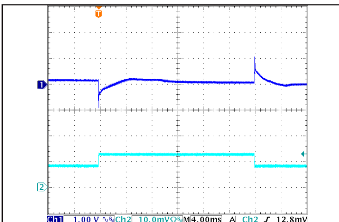
Figure 5: Output Voltage Response to Step-Change in Load Current (50% -75% -50% of I out (max); dI/dt = 0.1 A/μs). Load cap: 100 μF electrolytic cap and 1 μF ceramic cap. Ch 1: V out (1.00 V/div), Ch 2: I out (5.00 A/div). Timescale: 4.00 ms/div.
