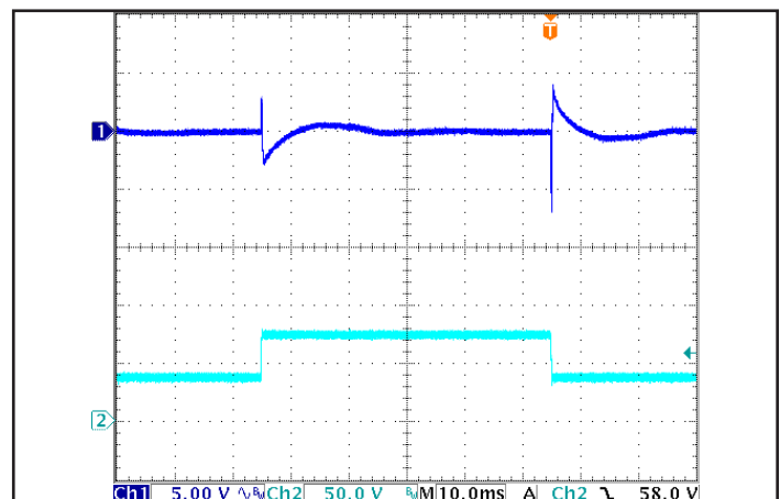
Figure 6: Output Voltage Response to Step-Change in Input Voltage (250 V/ms), at Max. load current. Load cap: 330 μF tantalum cap and 1 μF ceramic cap. Ch 1: V out (5.00 V/div), Ch 2: V in (50.0 V/div). Timescale: 10.0 ms/div.
