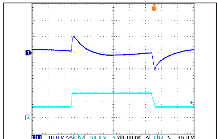
Figure 6: Output Voltage Response to Step-Change in Input Voltage (250 V/ms), at Max. load current. Load cap: 330 μF electrolytic cap and 1 μF ceramic cap. Ch 1: Vout (10.0 V/div), Ch 2: Vin (50.0 V/div). Timescale: 4.00 ms/div.
