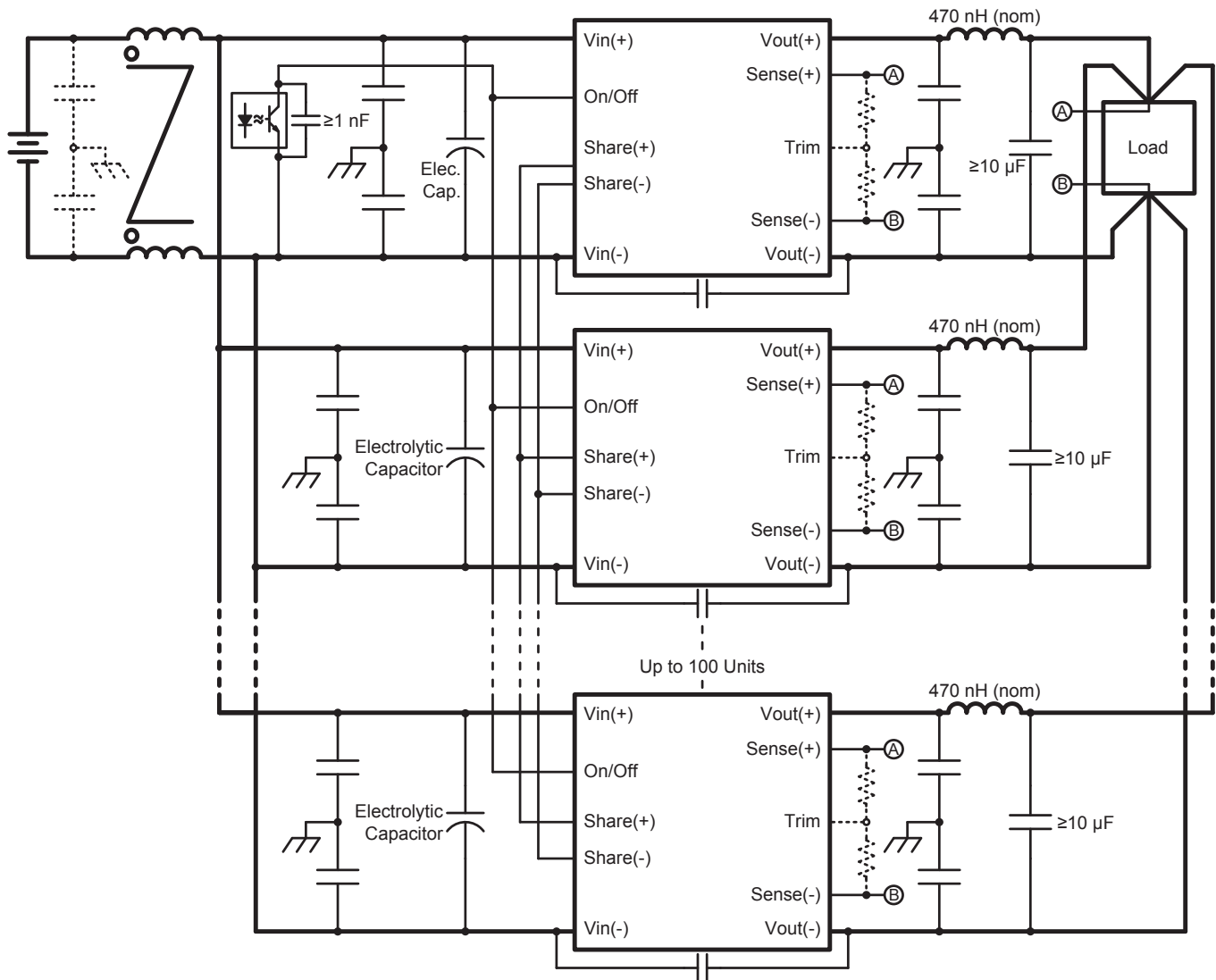
Figure E: Typical Application Circuit for Paralleling of Full-Featured Units with an Input Common-Mode Choke. If an input common-mode choke is used, Vin(-) MUST be tied together AFTER the choke for all units. 470 nH (nominal) inductor or an output common-mode choke is required for outputs >18 V. See Figure F for output common-mode choke configuration.
