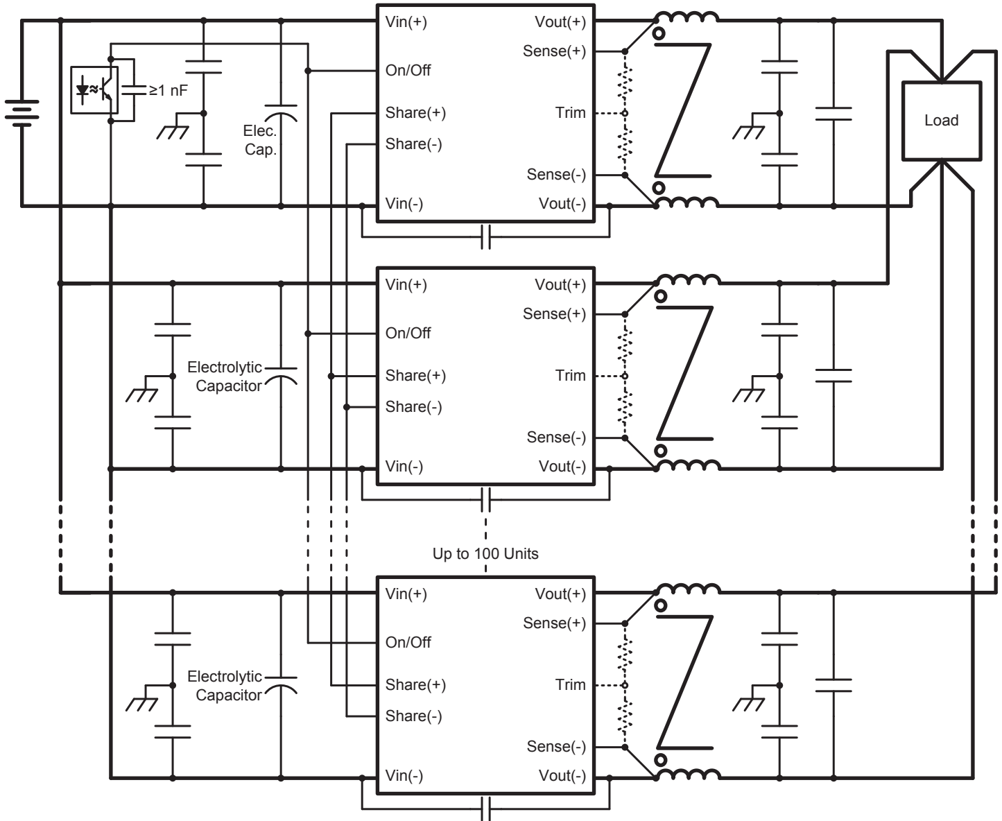
Figure F: Typical Application Circuit for Paralleling of Full-Featured Units with an Output Common-Mode Choke. When using an output common-mode choke, SENSE lines must be connected on the module-side of the choke. See Figure E for configuration with an input common-mode choke.
