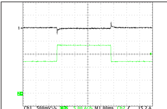
Figure 5: Output voltage response in the QT version to step-change in load current (50% - 75% - 50% of Iout(max); dI/dt = 0.1 A/μs). Load cap: 15 μF tantalum cap and 1 μF ceramic cap. Ch 1: Vout 500 mV/div, Ch 2: Iout 5 A/div.
