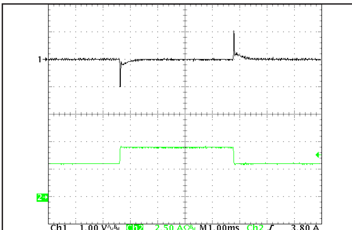
Figure 5: Output voltage response in the QT version to step-change in load current (50% - 75% - 50% of I out (max); dI/dt = 0.1 A/μs). Load cap: 15 μF tantalum cap and 1 μF ceramic cap. Ch 1: V out 1 V/div, Ch 2: I out 2.5 A/div.
