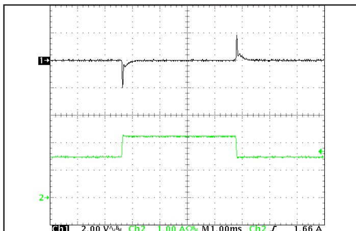
Figure 5: Output voltage response to step-change in load current (50 % -75 % -50 % of I out (max); dI/dt = 0.1 A/μs). Load cap: 15 μF tantalum cap and 1 μF ceramic cap. Ch 1: V out 2 V/div; Ch 2: I out 1 A/div.
