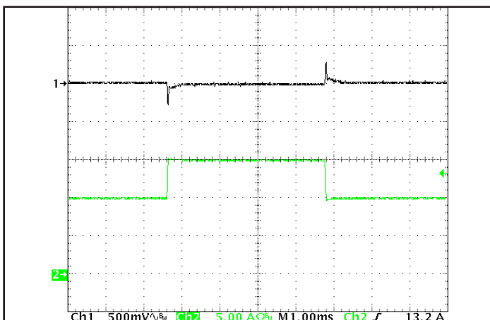
Figure 5: Output voltage response to step-change in load current (50 % -75 % -50 % of Iout(max); dI/dt = 0.1 A/μs). Load cap: 15 μF tantalum cap and 1 μF ceramic cap. Ch 1: Vout 500 mV/div; Ch 2: Iout 5 A/div.
