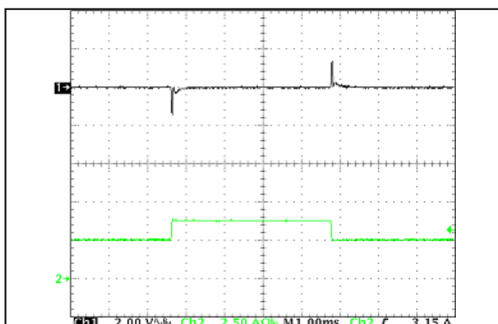
Figure 5: Output voltage response to step-change in load current (50 %-75 % -50 % of I out (max); dI/dt = 0.1 A/μs). Load cap: 15 μF tantalum cap and 1 μF ceramic cap. Ch 1: V out 2 V/div; Ch 2: I out 2.5 A/div.
