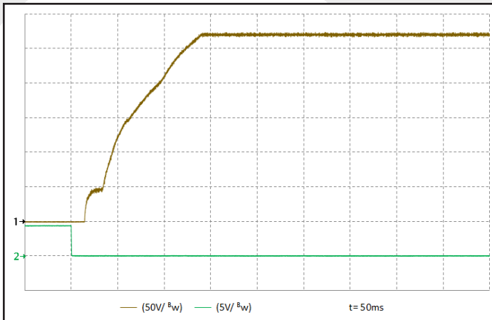
Figure 9: Turn-on transient at half resistive load and 47 \mu\text{F} output capacitance initiated by ENA. Input voltage pre-applied. Ch 1: Vout (50 V/div). Ch 2: ENA (5 V/div).
