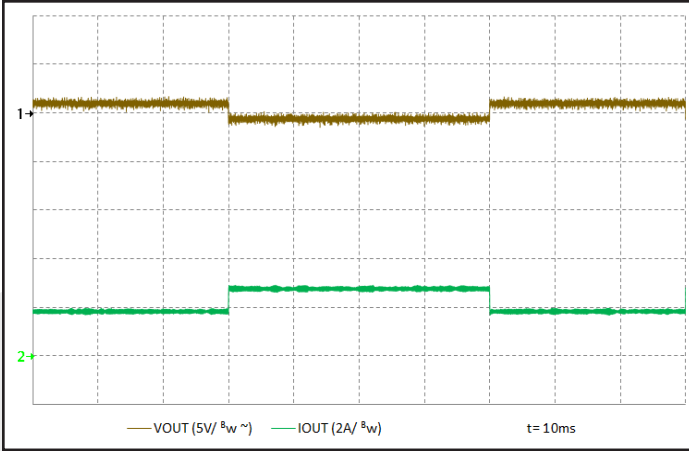
Figure 13: Output voltage response to step-change in load current 50%-75%-50% of I_{OUT(max)} . Ch 1: V_{OUT} (5V/div) Ch 2: I_{OUT} (2A/div). Plot created using measured V_{OUT} - V_{IN}/Turns Ratio
