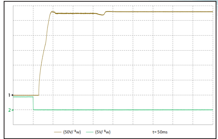
Figure 8: Turn-on transient at no load and 10 \mu\text{F} output capacitance initiated by ENA. Input voltage pre-applied. Ch 1: Vout (50 V/div). Ch 2: ENA (5 V/div).
