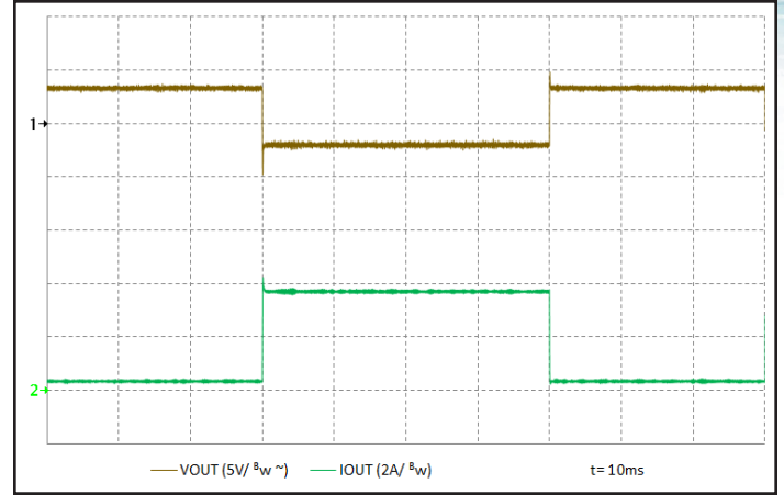
Figure 14: Output voltage response to step-change in load current 10%-100%-10% of I_{OUT(max)} . Ch 1: V_{OUT} (5 V/div). Ch 2: I_{OUT} (2 A/div). Plot created using measured V_{OUT} - V_{IN}/Turns Ratio
