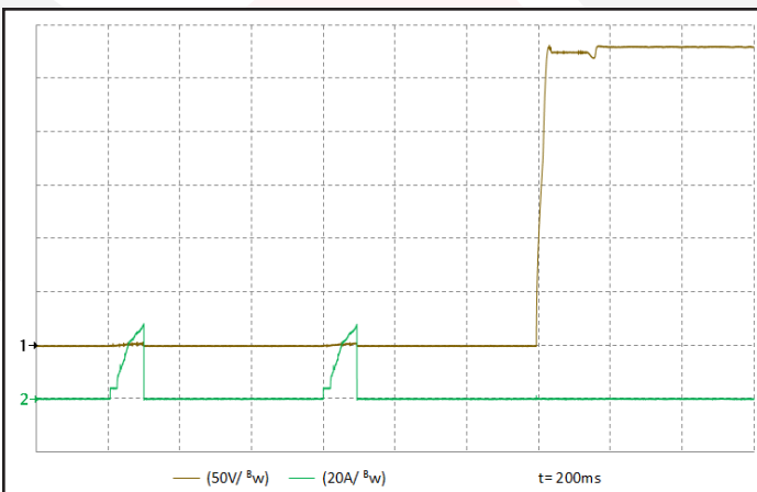
Figure 17: Rise of output voltage after the removal of a short circuit across the output terminals at 10 \mu F . R_{short} = 5 m\Omega . Ch 1: V_{OUT} (50 V/div). Ch 2: I_{OUT} (20 A/div). Bandwidth: 20MHz.
