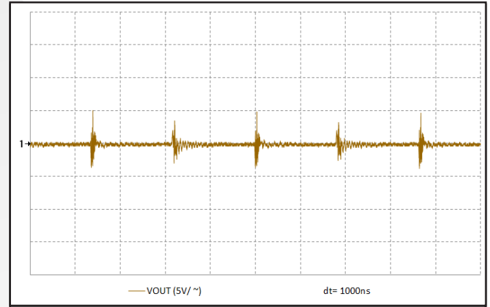
Figure 16: Output voltage ripple, V_{OUT} , at nominal input voltage and full load (5V/div). Bandwidth: Full. See Figure 12.
