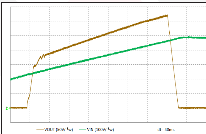
Figure 11: Turn-on and Turn-off behavior as a function of V_{in} . ENA previously enabled. Ch 1: Vout (50 V/div). Ch 2: Vin (100 V/div).
