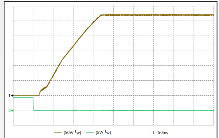
Figure 10: Turn-on transient at half resistive load and 423 \mu\text{F} output capacitance initiated by ENA. Input voltage pre-applied. Ch 1: Vout (50 V/div). Ch 2: ENA (5 V/div).
