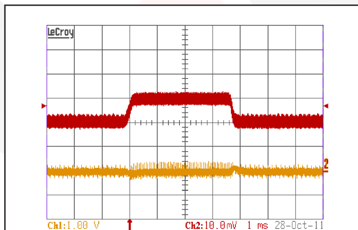
Figure 11: Output voltage response to step-change in load current (50%-75%-50% of I_{out(max)} ; dI/dt = 0.1 A/\mu s ). Load cap: 1 μF ceramic and 15 μF tantalum capacitors. Ch 1: Vout (1V/div), Ch 2: I_{out} (20A/div).
