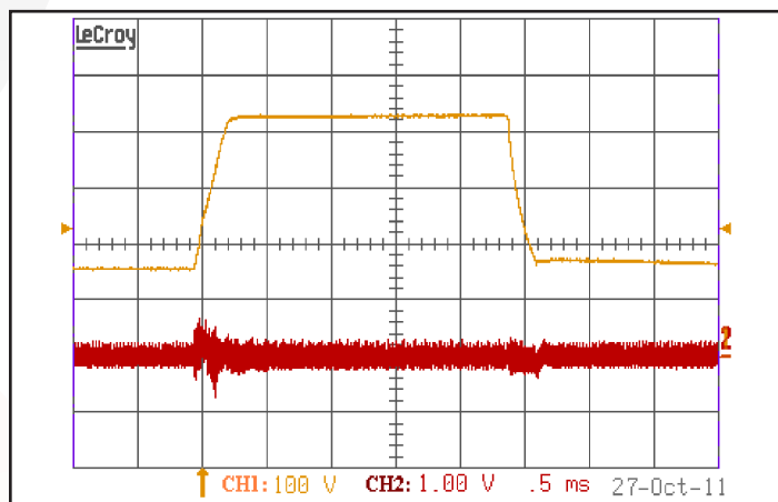
Figure 12: Output voltage response to step-change in input voltage (250V/ms). Load cap: 100 μF electrolytic output capacitance. Ch 1: Vin (100V/div), Ch 2: Vout (1V/div).
