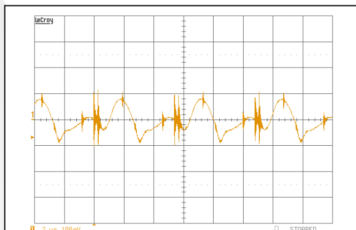
Figure 10: Output voltage ripple, V_{out} , at nominal input voltage and rated load current (100 mV/div). Load capacitance: 1μF ceramic capacitor and 10μF tantalum capacitor. Bandwidth: 25 MHz. See Figure 17.
