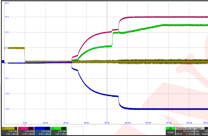
Figure 13: Turn-on transient at full load ( \pm 15 V and +5 V) and zero output capacitance initiated by On/Off. Nominal input voltage pre-applied. C1: On/Off (5 V/div); C2: +15 Vout (5 V/div); C3: -15 Vout (5 V/div); C4: +5 Vout (2 V/div); Timescale: 20 ms/div;
