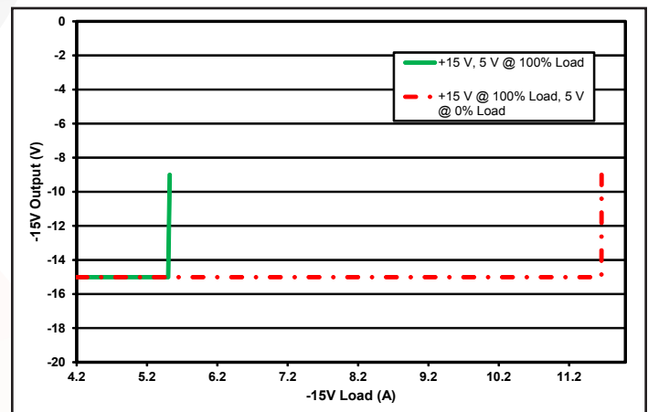
Figure 6: Output voltage vs. load current for -15\text{ V} output showing typical current limit curves at nominal input voltage.
