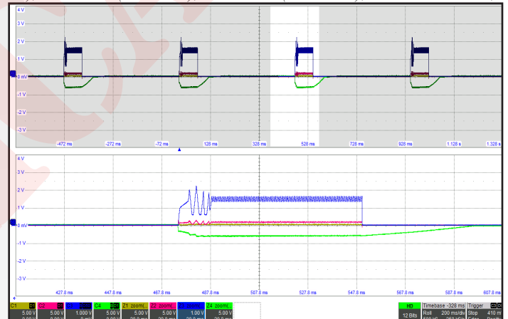
Figure 22: Load current vs. time with short circuit across +15 Vout terminals. Nominal input voltage applied. C1: +15 Vout (5 V/div); C2: -15 Vout (5 V/div); C3: +15 Iout (1 V = 50 A); C4: +5 Vout (5 V/div); Timescale: 20 ms/div;
