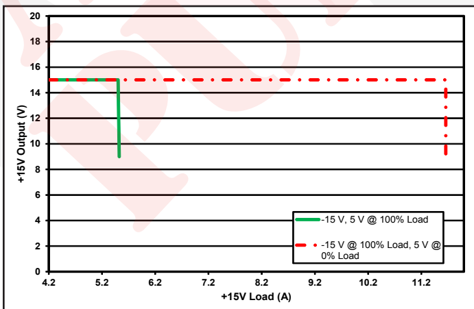
Figure 5: Output voltage vs. load current for +15\text{ V} output showing typical current limit curves at nominal input voltage.
