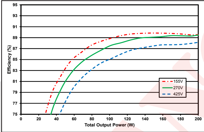
Figure 1: Efficiency vs. output power, from zero load to full load on the \pm 15\text{ V} output and the +5\text{ V} output at minimum, nominal, and maximum input voltage at 25^\circ\text{C} .
