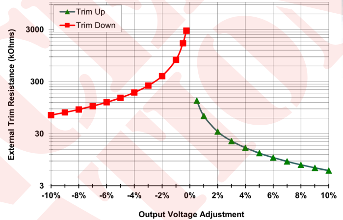
Figure B: Trim up and Trim down for 15 V output as a function of external trim resistance.
