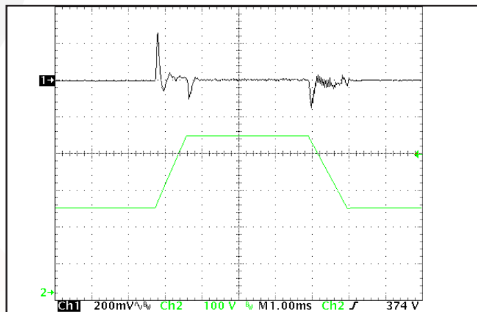
Figure 12: Output voltage response to step-change in input voltage (250V/ms). Load cap: 1μF ceramic and 15μF tantalum capacitors. Ch 1: Vout (200mV/div), Ch 2: Vin (100V/div), (1ms/div).
