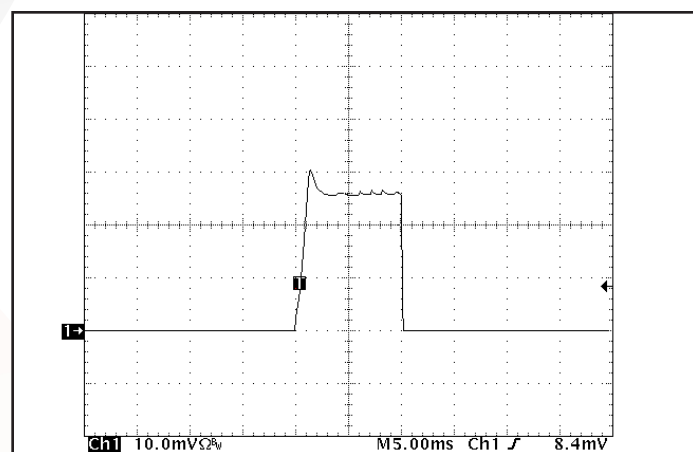
Figure 18: Load current (20A/div) as a function of time (5ms/div) when the converter attempts to turn on into a 10 m Ohm short circuit.
