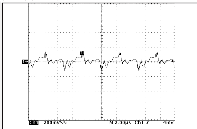
Figure 10: Output voltage ripple, Vout, at nominal input voltage and rated load current (200 mV/div), (2μs/div). Load capacitance: 1μF ceramic capacitor and 15μF tantalum capacitor. Bandwidth: 10 MHz. See Figure 17.
