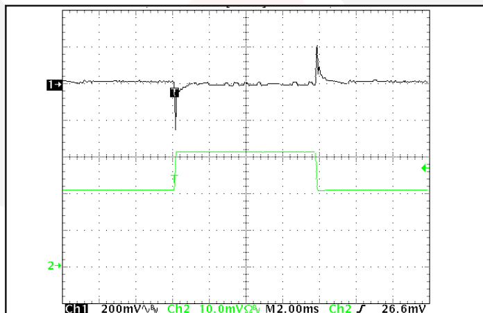
Figure 11: Output voltage response to step-change in load current (50%-75%-50% of I_{out(max)} ); ( dI/dt = 0.1 A/\mu s ). Load cap: 1 μF ceramic and 15 μF tantalum capacitors. Ch 1: Vout (200mV/div), Ch 2: I_{out} (10A/div), (2ms/div).
