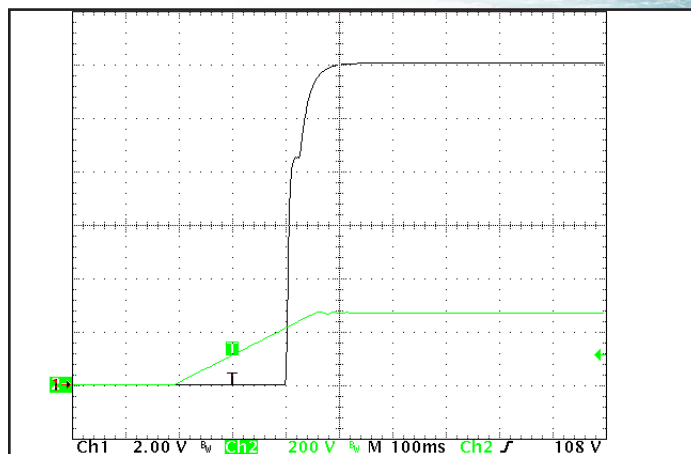
Figure 8: Turn-on transient at full resistive load and zero output capacitance initiated by Vin. ON/OFF Pin previously low. Ch 1: Vout (2V/div). Ch 2: Vin (200V/div), (100ms/div).
