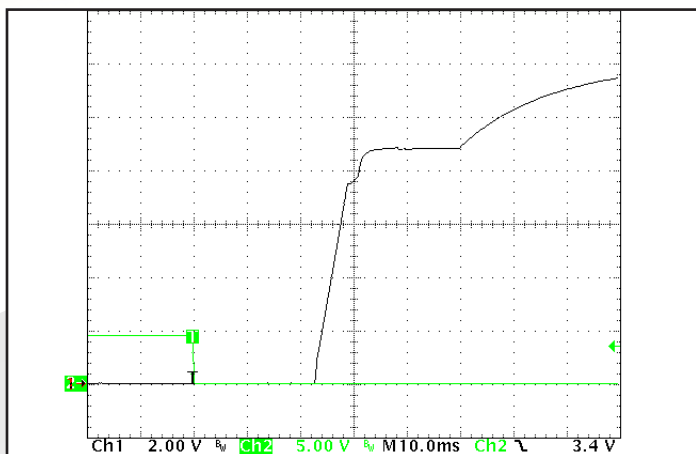
Figure 7: Typical startup waveform. Input voltage pre-applied, ON/OFF Pin on Ch 2, (10ms/div).
