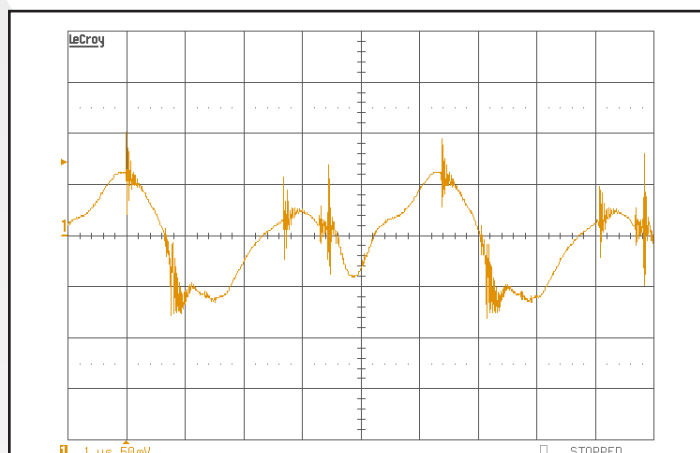
Figure 10: Output voltage ripple, V_{out} , at nominal input voltage and rated load current (50 mV/div). Load capacitance: 1µF ceramic capacitor and 10µF tantalum capacitor. Bandwidth: 25 MHz. See Figure 17.
