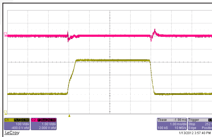
Figure 12: Output voltage response to step-change in input voltage (250V/ms). Load cap: 100 µF electrolytic output capacitance. Ch 1: V_{in} (100 V/div), Ch 2: V_{out} (1 V/div).
