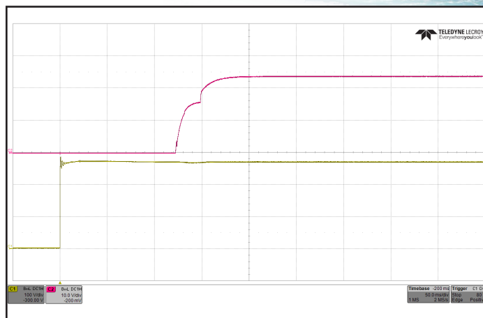
Figure 8: Turn-on transient at full resistive load and zero output capacitance initiated by V_{in} . ON/OFF Pin previously low. Ch 1: V_{in} (100V/div). Ch 2: V_{out} (10V/div). Timescale: 50.0ms/div.
