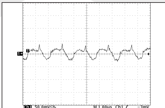
Figure 9: Input terminal current ripple, i_C , at full rated output current and nominal input voltage with SynQor MCOTS filter module (50 mA/div). Bandwidth: 20MHz. Timescale: 1.00µs/div. See Figure 17.
