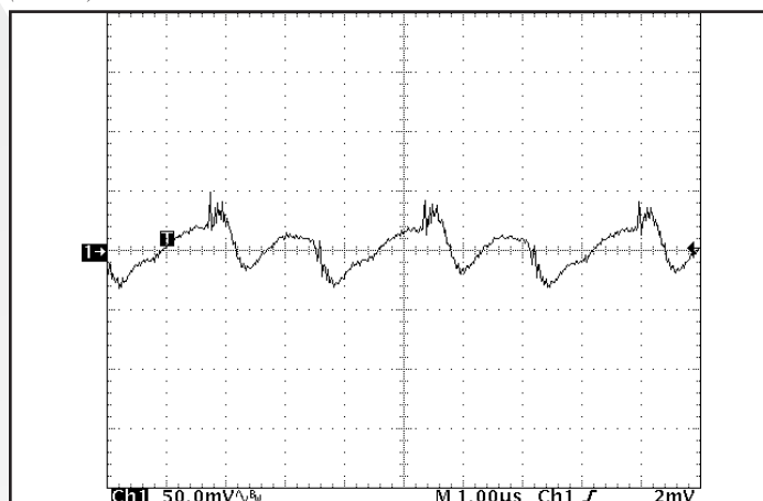
Figure 10: Output voltage ripple, V_{out} , at nominal input voltage and rated load current (50 mV/div). Load capacitance: 1µF ceramic capacitor and 15µF tantalum capacitor. Bandwidth: 20MHz. Timescale: 1.00µs/div. See Figure 17.
