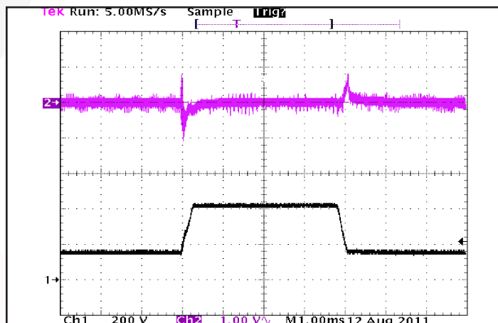
Figure 12: Output voltage response to step-change in input voltage (1000V/ms). Load cap: 100 μF electrolytic output capacitance. Ch 1: V_{in} (200V/div), Ch 2: V_{out} (1V/div).
