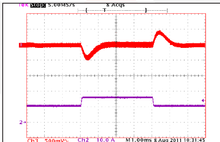
Figure 11: Output voltage response to step-change in load current (50%-75%-50% of I_{out(max)} ; dI/dt = 0.1 \text{ A}/\mu\text{s} ). Load cap: 1 μF ceramic and 15 μF tantalum capacitors. Ch 3: V_{out} (500mV/div), Ch 2: I_{out} (10A/div).
