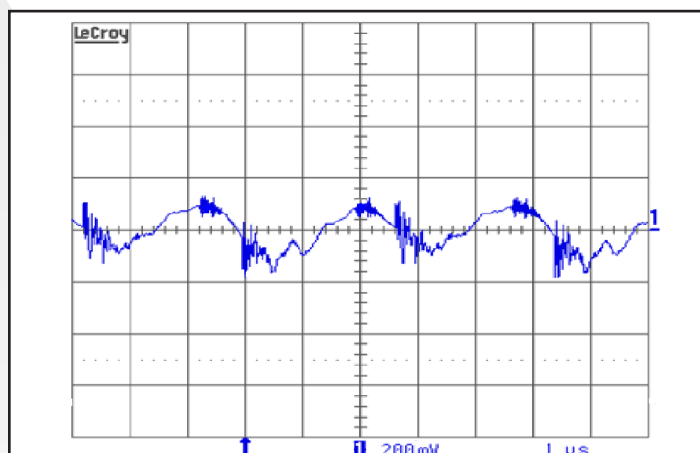
Figure 10: Output voltage ripple, V_{out} , at nominal input voltage and rated load current (200 mV/div). Load capacitance: 1μF ceramic capacitor and 10μF tantalum capacitor. Bandwidth: 25 MHz. See Figure 17.
