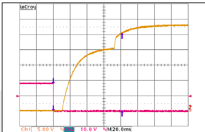
Figure 7: Start waveform with 1% load. Input voltage pre-applied, ON/OFF Pin on Ch 2.
