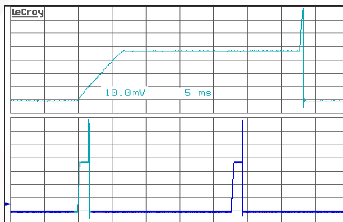
Figure 18: Load current (10A/div) as a function of time (5ms/div and 100ms/div) when the converter attempts to turn on into a 10 mΩ short circuit.
