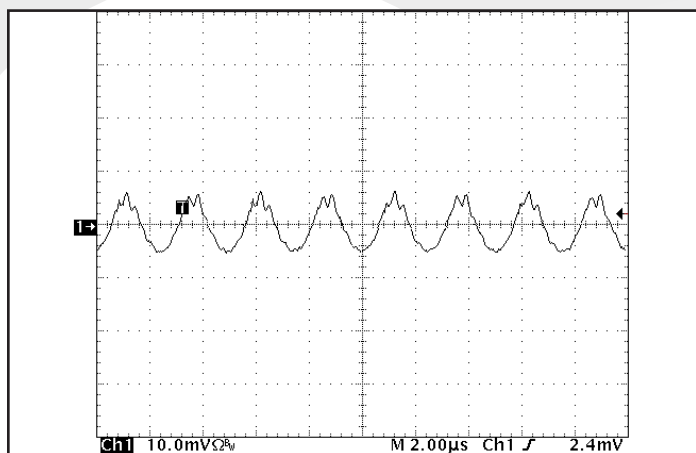
Figure 9: Input terminal current ripple, i_C , at full rated output current and nominal input voltage with 10\mu H source impedance and 10\mu F electrolytic capacitor (200mA/div), (2μs/div). Bandwidth: 20MHz. See Figure 17.
