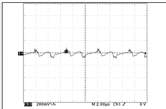
Figure 10: Output voltage ripple, 28Vout, at nominal input voltage and rated load current (200 mV/div), (2μs/div). Load capacitance: 1\mu F ceramic capacitor and 15\mu F tantalum capacitor. Bandwidth: 10 MHz. See Figure 17.
