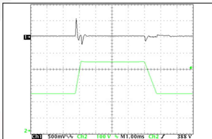
Figure 12: Output voltage response to step-change in input voltage (250V/ms). Load cap: 1\mu F ceramic and 15\mu F tantalum capacitors. Ch 1: Vout (500mV/div), Ch 2: Vin (100V/div), (1ms/div).
