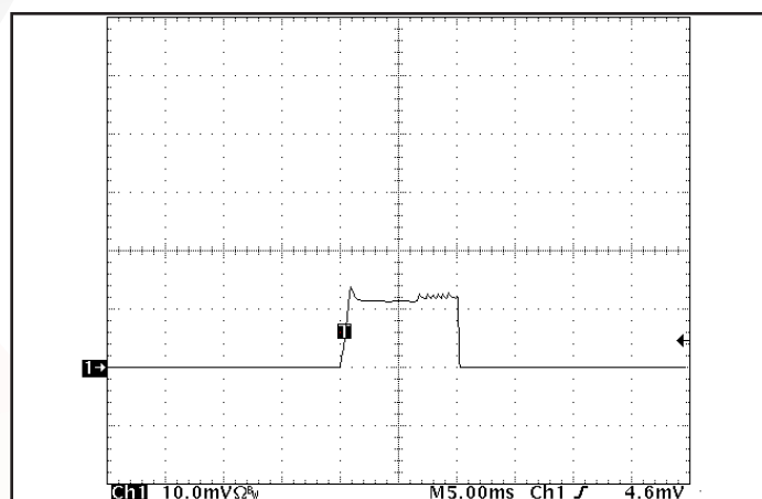
Figure 18: Load current (20A/div) as a function of time (5ms/div) when the converter attempts to turn on into a 10 m \Omega short circuit.
