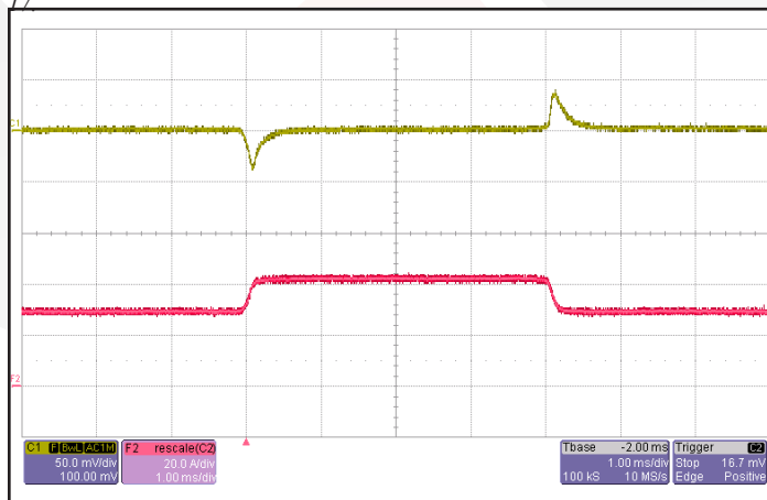
Figure 11: Output voltage response to step-change in load current (50%-75%-50% of I_{out(max)} ; dI/dt = 0.1 A/μs ). Load cap: 1 μF ceramic and 15 μF tantalum capacitors. Ch 1: V_{out} (50mV/div), Ch 2: I_{out} (20A/div). Timescale: 1.00ms/div.
