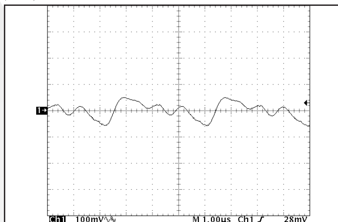
Figure 10: Output voltage ripple, V_{out} , at nominal input voltage and rated load current (100 mV/div). Load capacitance: 1μF ceramic capacitor and 15μF tantalum capacitor. Bandwidth: 10 MHz. Timescale: 1.00μs/div. See Figure 17.
