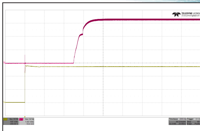
Figure 8: Turn-on transient at full resistive load and zero output capacitance initiated by Vin. ON/OFF Pin previously low. Ch 1: Vin (100V/div). Ch 2: Vout (1V/div). Timescale: 50ms/div.
