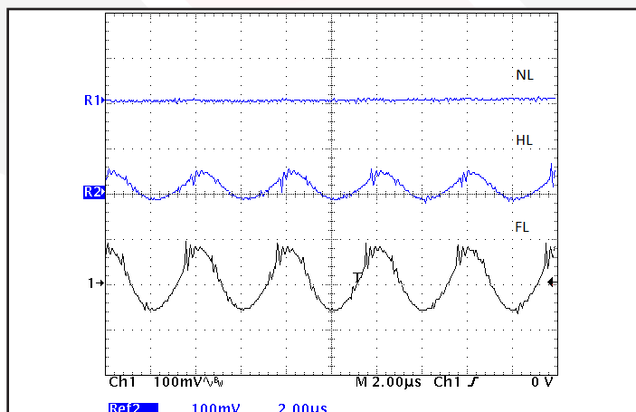
Figure 11: Output Voltage Ripple, 28Vout, at nominal input voltage and rated load current. Load capacitance: 1μF ceramic capacitor and 15μF tantalum capacitor. Bandwidth: 10MHz. See Figure 17. Ch 1: Vout (100mV/div), Time (2μs/div).
