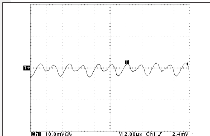
Figure 10: Input Terminal Current Ripple, i_c , at full rated output current and nominal input voltage. Bandwidth: 2MHz. See Figure 17. Ch 1: i_c (200mA/div), Time (2μs/div).
