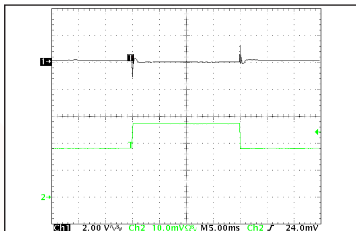
Figure 12: Output voltage response to step-change in load current (500W-750W-500W; di/dt = 0.1A/\mu S ). Load cap: 1μF ceramic and 15μF tantalum capacitors. Ch 1: Vout (2V/div), Ch 2: Iout (10A/div), Time (ms/div).
