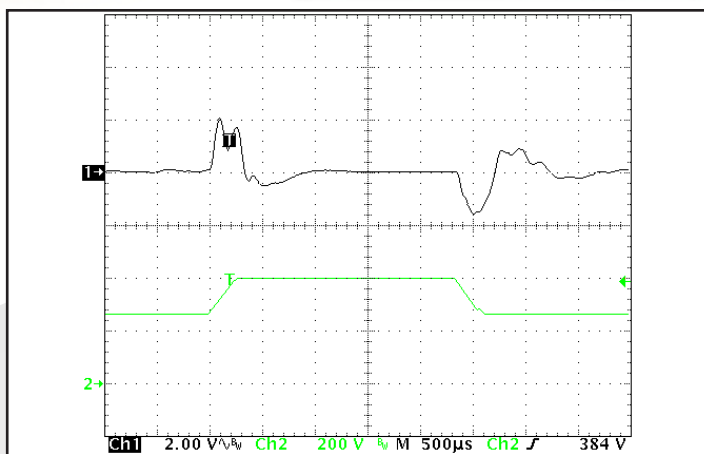
Figure 13: Output voltage response to step-change in input voltage (250V/ms). Load cap: 100 \mu F electrolytic output capacitance. Ch 1: Vout (2V/div), Ch 2: Vin (200V/div). Time (500 \mu S/div).
