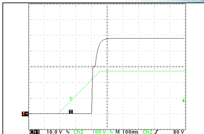
Figure 8: Turn-on transient at full resistive load and zero output capacitance initiated by Vin. ON/OFF Pin previously low. Ch 1: Vout (10V/div). Ch 2: Vin (100V/div), (100ms/div).
