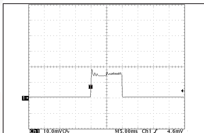
Figure 18: Load current (10A/div) as a function of time (5ms/div) when the converter attempts to turn on into a 10 mΩ short circuit.
