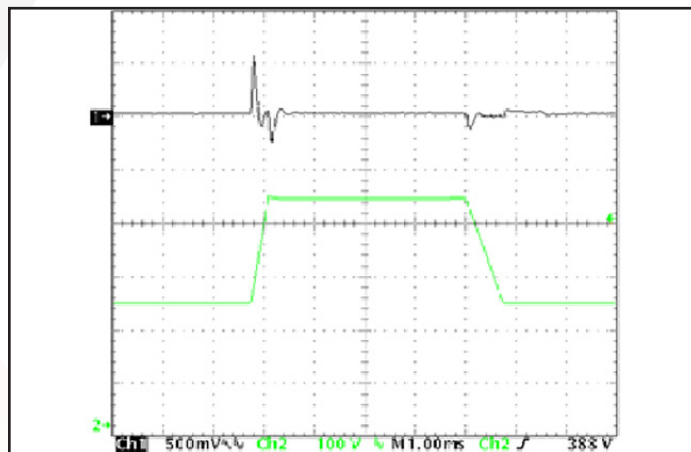
Figure 12: Output voltage response to step-change in input voltage (250V/ms). Load cap: 1μF ceramic and 15μF tantalum capacitors. Ch 1: Vout (500mV/div), Ch 2: Vin (100V/div), (1ms/div).
