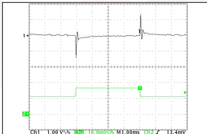
Figure 11: Output voltage response to step-change in load current (50%-75%-50% of I_{out(max)} ); ( dI/dt = 0.1 A/μs ). Load cap: 1 μF ceramic and 15 μF tantalum capacitors. Ch 1: Vout (1V/div), Ch 2: I_{out} (5A/div), (1ms/div).
