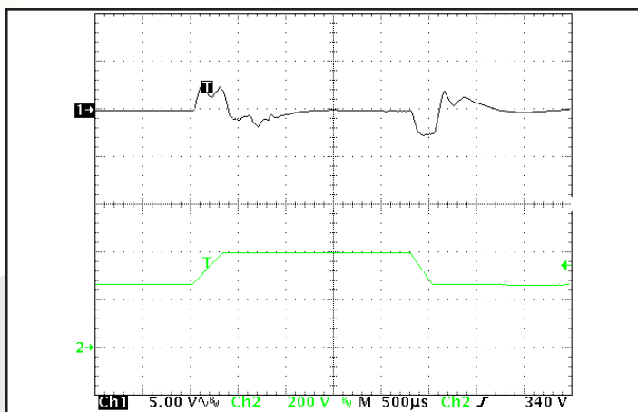
Figure 13: Output voltage response to step-change in input voltage (250V/ms). Load cap: 100 \mu F electrolytic output capacitance. Ch 1: V_{out} (5V/div), Ch 2: V_{in} (200V/div), Time (500 \mu S/div).
