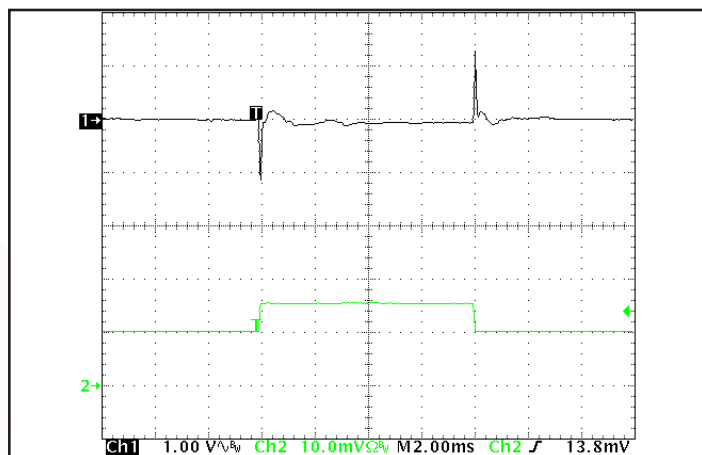
Figure 12: Output voltage response to step-change in load current (500W-750W-500W); di/dt = 0.1 \text{ A}/\mu\text{s} . Load cap: 1 μF ceramic and 15 μF tantalum capacitors. Ch 1: Vout (1V/div), Ch 2: Iout (10A/div), Time (2ms/div).
