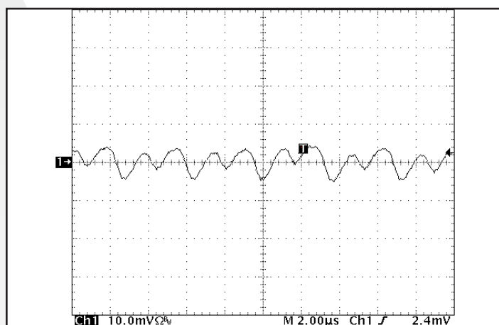
Figure 10: Input terminal current ripple, i_c at full rated output current and nominal input voltage. Bandwidth: 20MHz. See Figure 17. Ch 1: i_c (200 mA/div), Time (2μs/div).
