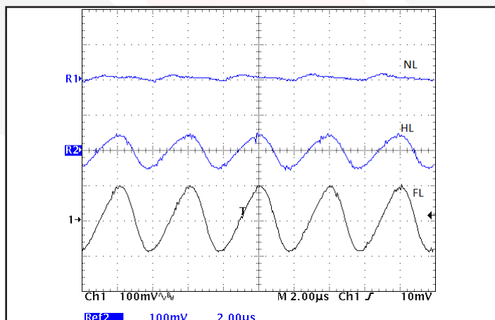
Figure 11: Output voltage ripple, 28Vout, at nominal input voltage and rated load current. Load capacitance: 1μF ceramic capacitor and 15μF tantalum capacitor. Bandwidth: 10 MHz. See Figure 17. Ch 1: Vout (100 mV/div), Time (2μs/div).
