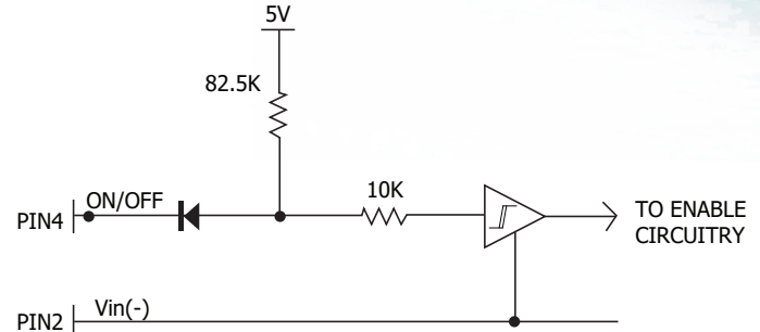
Figure A: Circuit diagram shown for reference only, actual circuit components may differ from values shown for equivalent circuit.
