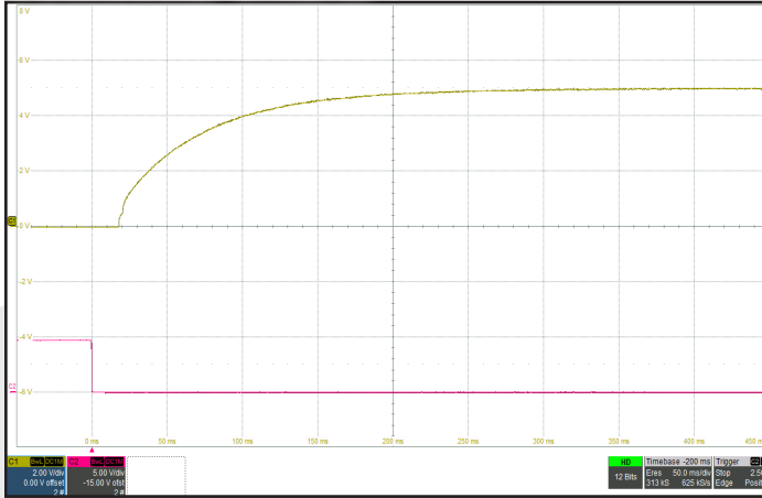
Figure 7: Turn-on transient at no load and zero output capacitance initiated by On/Off. Input voltage pre-applied. Ch 1: Vout (2 V/div). Ch 2: On/Off (5 V/div). Timescale: 50.0ms/div.
