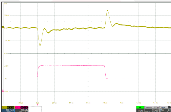
Figure 11: Output voltage response to step-change in load current 50%-100%-50% of Iout (max). No external load capacitance. Ch 1: Vout (500 mV/div). Ch 2: Iout (2 A/div). Timescale: 200μs/div.
