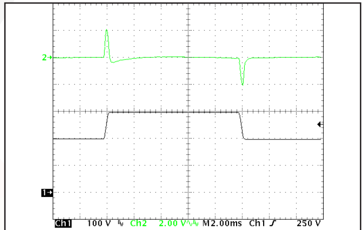
Figure 12: Output voltage response to step-change in input voltage (200 V - 300 V - 200 V); dV/dt = 400 V/ms. Ch 1: Vin (100 V/div). Ch 2: Vout (2 V/div). (2 ms/div).
