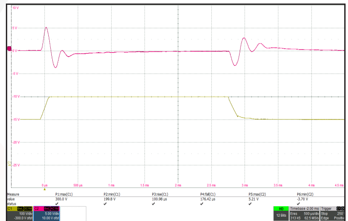
Figure 12: Output voltage response to step-change in input voltage (200 V - 300 V - 200 V) in 150 μs. Ch 2: Vout (5 V/div). Ch 1: Vin (100 V/div). Timescale: 500μs/div.
