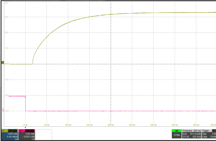
Figure 7: Turn-on transient at no load and zero output capacitance initiated by On/Off. Input voltage pre-applied. Ch 1: Vout (1 V/div). Ch 2: On/Off (5 V/div). Timescale: 50.0ms/div.
