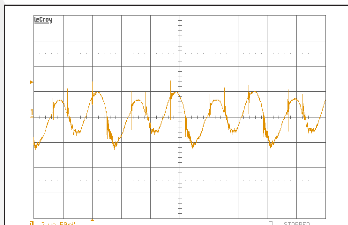
Figure 10: Output voltage ripple, Vout, at nominal input voltage and rated load current (50 mV/div). Load capacitance: 10μF tantalum capacitor. Bandwidth: 20 MHz. See Figure 17.
