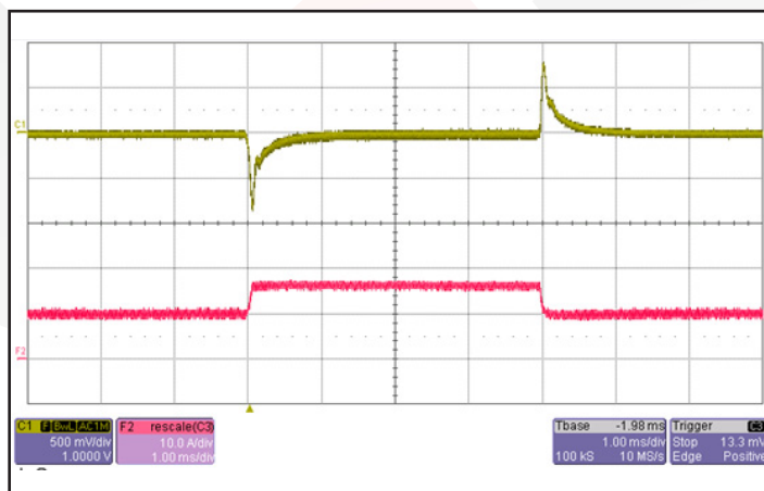
Figure 11: Output voltage response to step-change in load current (50%-75%-50% of Iout(max); dI/dt = 0.1 A/μs). Load cap: 1 μF ceramic and 15 μF tantalum capacitors. Ch 1: Vout (500mV/div), Ch 2: Iout (10A/div).
