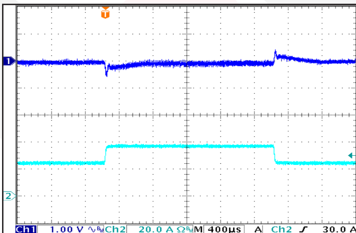
Figure 11: Output voltage response to step-change in load current (50%-75%-50% of I_{out(max)} ; dI/dt = 5 \text{ A}/\mu\text{s} ). Load cap: 1µF ceramic and 100µF electrolytic capacitors. Ch 1: Vout (1V/div), Ch 2: Iout (20A/div). Timescale: 400µs/div.
