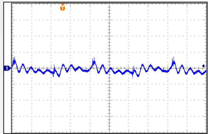
Figure 10: Output voltage ripple, Vout, at nominal input voltage and rated load current (100 mV/div). Load capacitance: 1µF ceramic capacitor and 100µF electrolytic capacitor. Bandwidth: 20 MHz. Timescale: 2.00µs/div. See Figure 13.
