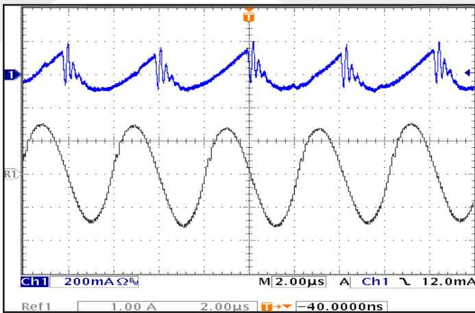
Figure 9: Input terminal current ripple, i_c , at full rated output current with 470µF electrolytic capacitance. Ch 1: 28 Vin (200mA/div), Ref1: 50 Vin (1A/div). Bandwidth: 20MHz. Timescale: 2.00µs/div. See Figure 13.
