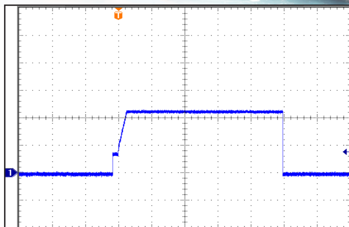
Figure 14: Output Short Load Current , (2 A/div) as a function of time (40 ms/div) when the converter attempts to turn on into a 10 mΩ short circuit.
