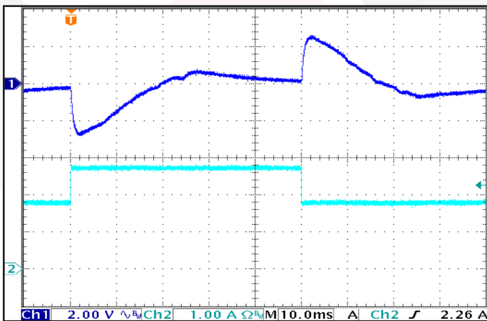
Figure 11: Output Voltage Response to Step-Change in Load Current , (50%-75%-50% of I_{out(max)} ; dI/dt = 5 A/ \mu s). Load capacitance: 1 \mu F ceramic and 100 \mu F electrolytic capacitors. Ch 1: \Delta V_{out} (2 V/div); Ch 2: I_{out} (1 A/div). Timescale: 10.0ms/div.
