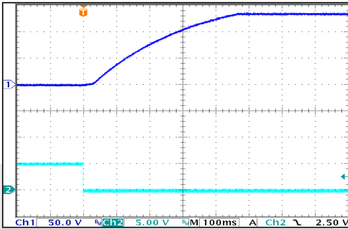
Figure 7: Typical Startup Waveform , input voltage pre-applied. Ch 1: V_{out} (50 V/div); Ch 2: ON/OFF Pin (5 V/div). Timescale: 100ms/div.
