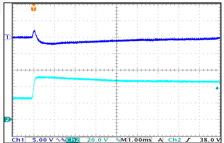
Figure 12: Output Voltage Response to Step-Change in Input Voltage , (250 V/ms). Load capacitance: 1 \mu F ceramic and 100 \mu F electrolytic capacitors. Ch 1: \Delta V_{out} (5 V/div); Ch 2: V_{in} (20 V/div). Timescale: 1.00ms/div.
