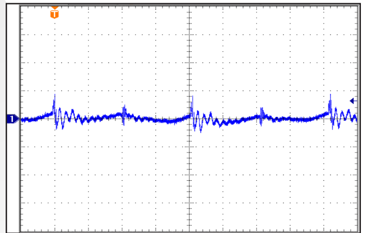
Figure 10: Output Voltage Ripple , V_{out} , at nominal input voltage and rated load current (100 mV/div). Load capacitance: 1 \mu F ceramic and 100 \mu F electrolytic capacitors. Bandwidth: 20 MHz. Timescale: 2.00 \mu s/div. See Figure 13.
