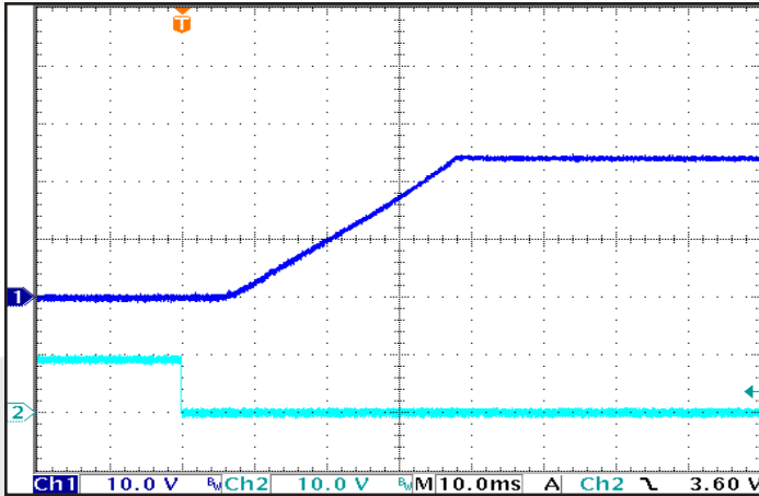
Figure 7: Typical Startup Waveform , input voltage pre-applied. Ch 1: V_{out} (10V/div); Ch 2: ON/OFF Pin (10V/div). Timescale: 10.0ms/div.
