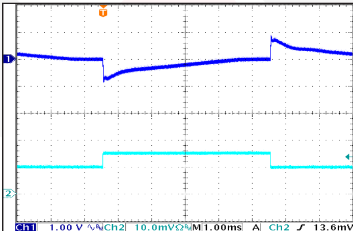
Figure 11: Output Voltage Response to Step-Change in Load Current , (50%-75%-50% of I_{out(max)} ; dI/dt = 5\text{A}/\mu\text{s} ). Load capacitance: 1 \mu\text{F} ceramic and 100 \mu\text{F} electrolytic capacitors. Ch 1: V_{out} (1V/div); Ch 2: I_{out} (10A/div). Timescale: 1.00ms/div.
