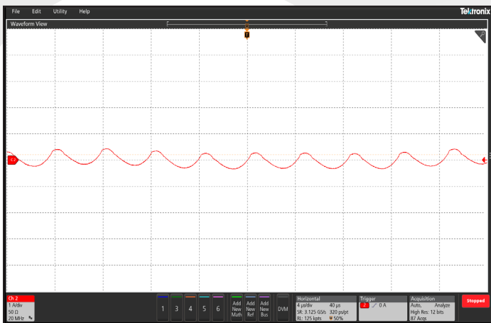
Figure 9: Input Terminal Current Ripple, i_C , at full rated output current and nominal input voltage with a 470 μF electrolytic capacitor (1 A/div); Timebase: 4 μs/div; Bandwidth: 20 MHz. See Figure 13.
