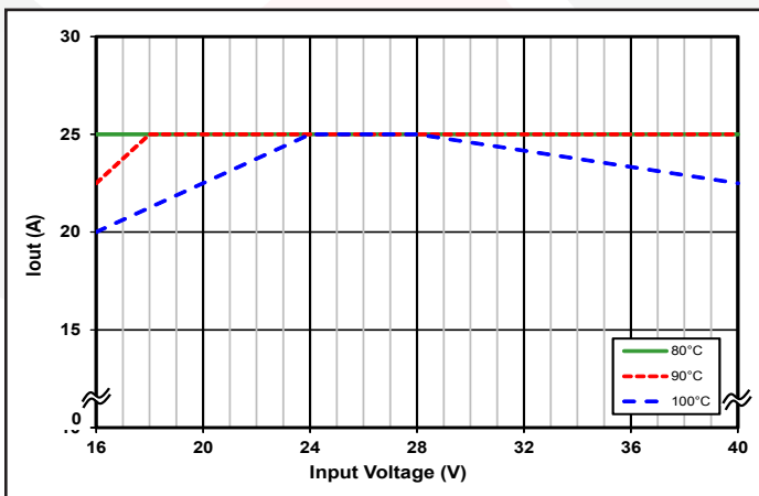
Figure 5: Thermal Derating, (maximum output current vs. continuous input voltage) at selected baseplate temperatures.
