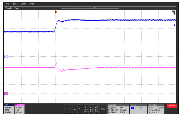
Figure 12: Output Voltage Response to Step-Change in Input Voltage, ( dV/dt = 250 V/ms ). Load capacitance: 1 μF ceramic. Ch 1: Vin (10 V/div); Ch 6: Vout (10 V/div). Timebase: 400 μs/div
