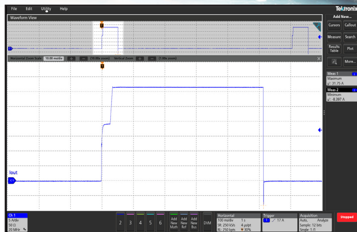
Figure 14: Output Short Load Current , (5A/div) as a function of time (10 ms/div, zoomed in) when the converter attempts to turn on into a 10 mΩ short circuit.
