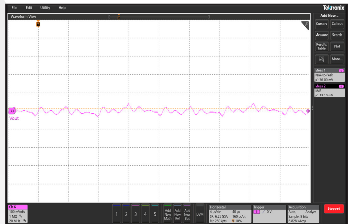
Figure 10: Output Voltage Ripple, Vout, at nominal input voltage and rated load current (100 mV/div). Load capacitance: 4 μF ceramic and 470 μF electrolytic capacitors. Timebase: 4 μs/div; Bandwidth: 20 MHz. See Figure 13.
