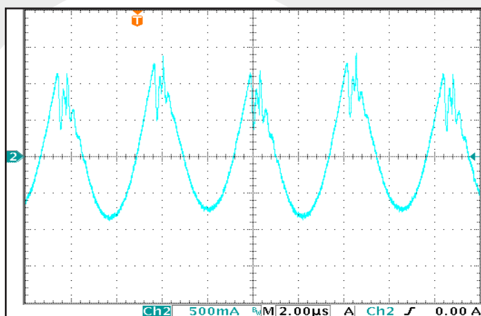
Figure 9: Input Terminal Current Ripple , i_{in} , at full rated output current and nominal input voltage with a 470 \mu F electrolytic capacitor (500 mA/div). Bandwidth: 20 MHz. Timescale: 2.00 \mu s/div. See Figure 13.
