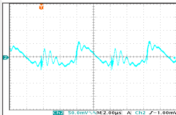
Figure 10: Output Voltage Ripple , Vout, at nominal input voltage and rated load current (50 mV/div). Load capacitance: 1 \mu F ceramic and 10 \mu F tantalum capacitors. Bandwidth: 20 MHz. Timescale: 2.00 \mu sec/div. See Figure 13.
