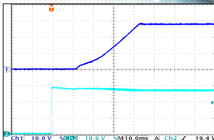
Figure 8: Turn-On Transient , at full resistive load and zero output capacitance, initiated by Vin. Ch 1: Vout (10 V/div); Ch 2: Vin (10 V/div). Timescale: 10.0ms/div.
