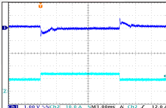
Figure 17: Hi-Cap Option Output Voltage Response to Step-Change in Load Current , (50%-75%-50% of Iout(max); dI/dt = 10 A/μs). Load capacitance: 1 μF ceramic and 100 μF electrolytic capacitors. Ch 1: ΔVout (1 V/div); Ch 2: Iout (10 A/div). Timescale: 1.00ms/div.
