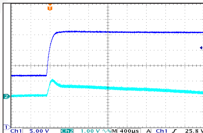
Figure 12: Output Voltage Response to Step-Change in Input Voltage , ( dV/dt = 250 V/ms). Load capacitance: 1 \mu F ceramic and 990 \mu F electrolytic capacitors. Ch 1: Vin (5 V/div); Ch 2: \Delta V_{out} (1 V/div). Timescale: 400 \mu s/div.
