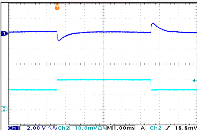
Figure 11: Output Voltage Response to Step-Change in Load Current , (50%-75%-50% of I_{out(max)} ; dI/dt = 5A/μs ). Load capacitance: 1μF ceramic and 100μF electrolytic capacitors. Ch 1: \Delta V_{out} (2 V/div); Ch 2: I_{out} (5 A/div). Timescale: 1.00ms/div.
