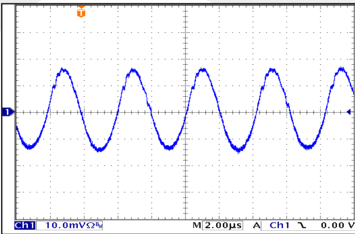
Figure 9: Input Terminal Current Ripple , i_C , at full rated output current and nominal input voltage with SynQor MCOTS filter module (0.5 A/div). Bandwidth: 20 MHz. Timescale: 2.00μs/div. See Figure 13.
