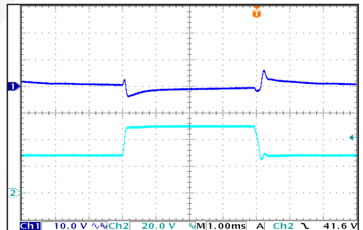
Figure 12: Output Voltage Response to Step-Change in Input Voltage , ( dV/dt = 250 V/ms ). Load capacitance: 1μF ceramic and 100μF electrolytic capacitors. Ch 1: Vout (10 V/div); Ch 2: \Delta V_{in} (20 V/div). Timescale: 1.00ms/div.
