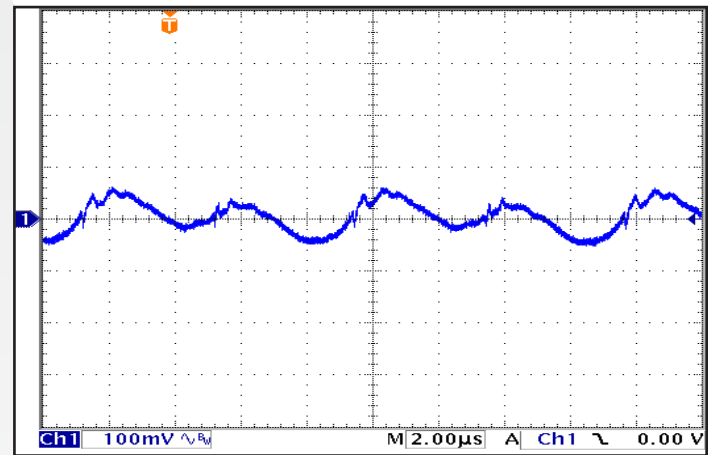
Figure 10: Output Voltage Ripple , Vout, at nominal input voltage and rated load current (100 mV/div). Load capacitance: 1μF ceramic and 100μF electrolytic capacitors. Bandwidth: 20 MHz. Timescale: 2.00μs/div. See Figure 13.
