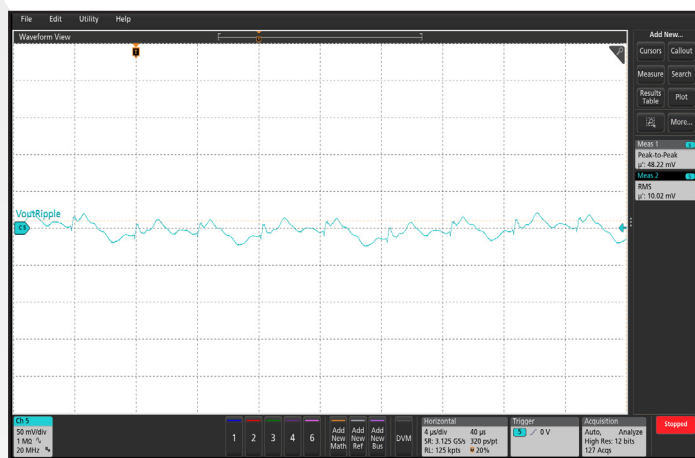
Figure 10: Output Voltage Ripple, Vout, at nominal input voltage and rated load current (50 mV/div). Load capacitance: 4 \mu F ceramic and 470 \mu F electrolytic capacitors. Timebase: 4 \mu s/div; Bandwidth: 20 MHz. See Figure 13.
