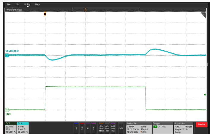
Figure 18: Hi-Cap Option Output Voltage Response to Step-Change in Load Current, (0%-100%-0% of I OUT (max); dI/dt = 10 A/µs). Load capacitance: 4 µF ceramic and 25 mF electrolytic capacitors. Ch 5: ΔVout (1 V/div); Ch 3: Iout (20 A/div); Timebase: 2 ms/div
