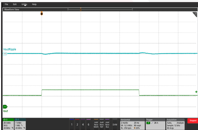
Figure 17: Hi-Cap Option Output Voltage Response to Step-Change in Load Current, (50%-75%-50% of I OUT (max); dI/dt = 10 A/µs). Load capacitance: 4 µF ceramic and 25 mF electrolytic capacitors. Ch 5: ΔVout (1 V/div); Ch 3: Iout (20 A/div); Timebase: 2 ms/div
