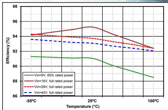
Figure 2: Efficiency, at nominal output voltage vs. case temperature for selected input voltages.
