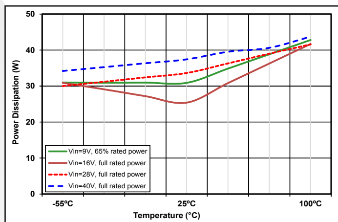
Figure 4: Power Dissipation, at nominal output voltage vs. case temperature for selected input voltages.
