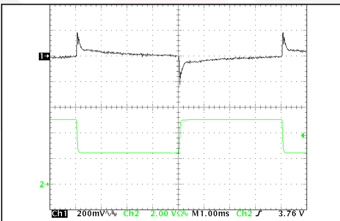
Figure 11: Output voltage response to step-change in load current 50%-100%-50% of Iout (max); dI/dt = 0.05 \text{ A}/\mu\text{s} . No external load capacitance. Ch 1: Vout (200 mV/div). Ch 2: Iout (2 A/div). (1 ms/div).
