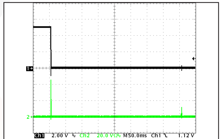
Figure 18: A short circuit across the output terminals. Ch 1: V_{out} (2 V/div). Ch 2: I_{out} (20 A/div). (50 ms/div).
