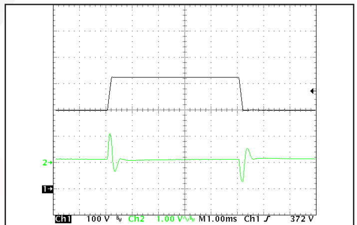
Figure 12: Output voltage response to step-change in input voltage (300 V - 425 V - 300 V); dV/dt = 800 \text{ V}/\text{ms} . Ch 1: Vin (100 V/div). Ch 2: Vout (1 V/div). (1 ms/div).
