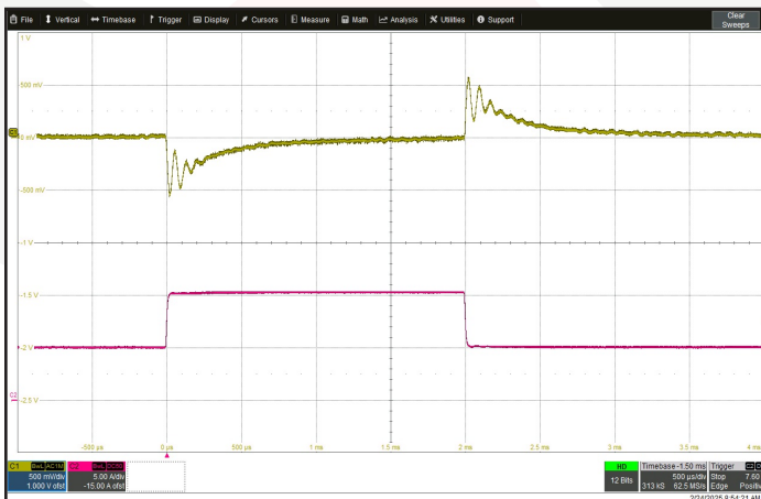
Figure 11: Output voltage response to step-change in load current 50%-100%-50% of I_{out(max)} . No external load capacitance. Ch 1: V_{out} (500 mV/div). Ch 2: I_{out} (5 A/div). Timescale: 500 \mu s/div.
