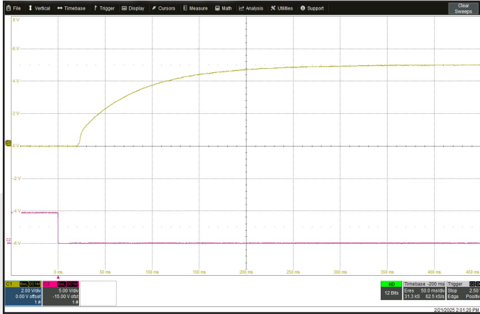
Figure 7: Turn-on transient at full load and zero output capacitance initiated by On/Off. Input voltage pre-applied. Ch 1: V_{out} (2 V/div). Ch 2: On/Off (5 V/div). Timescale: 50.0 ms/div.
