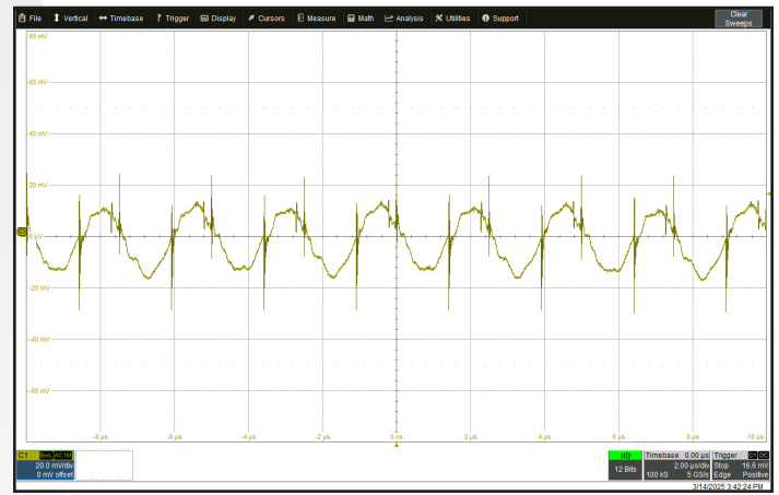
Figure 10: Output voltage ripple, V_{out} , at nominal input voltage and full rated load current (20 mV/div). Timescale: 2.00 \mu s/div.
