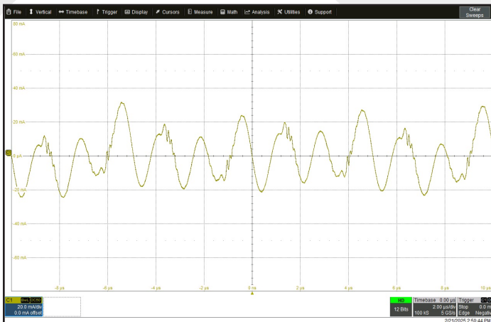
Figure 9: Input terminal current ripple, at full rated output current and nominal input voltage (20 mA/div). Timescale: 2.00 \mu s/div. See Figure 17.
