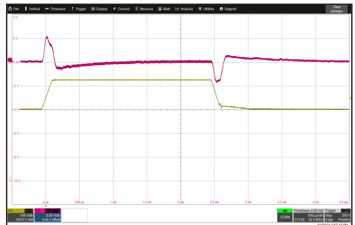
Figure 12: Output voltage response to step-change in input voltage (300 V - 425 V - 300 V) in 125 μs. Ch 1: V_{in} (100 V/div). Ch 2: V_{out} (2 V/div). Timescale: 500 μs/div.
