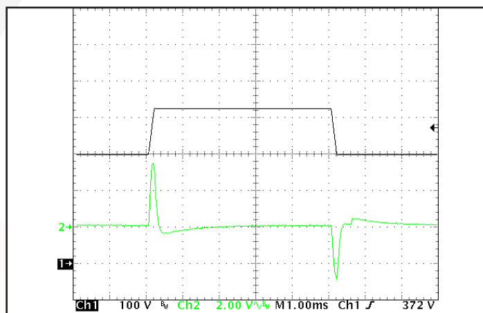
Figure 12: Output voltage response to step-change in input voltage (300 V - 425 V - 300 V); dV/dt = 800 \text{ V}/\text{ms} . Ch 1: Vin (100 V/div). Ch 2: Vout (2 V/div). (1 ms/div).
