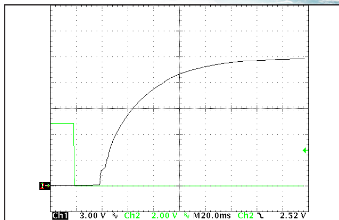
Figure 8: Turn-on transient at full resistive load and zero output capacitance initiated by On/Off. Input voltage pre-applied. Ch 1: Vout (3 V/div). Ch 2: On/Off (2 V/div). (20 ms/div).
