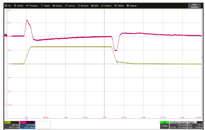
Figure 12: Output voltage response to step-change in input voltage (300 V - 425 V - 300 V) in 125 \mu s. Ch 1: V_{in} (100 V/div). Ch 2: V_{out} (2 V/div). Timescale: 500 \mu s/div.
