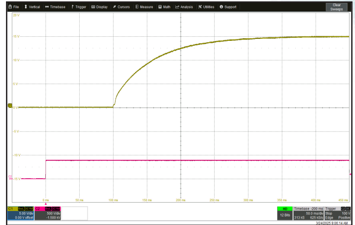
Figure 8: Turn-on transient at full load and zero output capacitance initiated by V_{in} . On/Off Pin previously low. Ch 1: V_{out} (5 V/div). Ch 2: V_{in} (500 V/div). Timescale: 50.0 ms/div.
