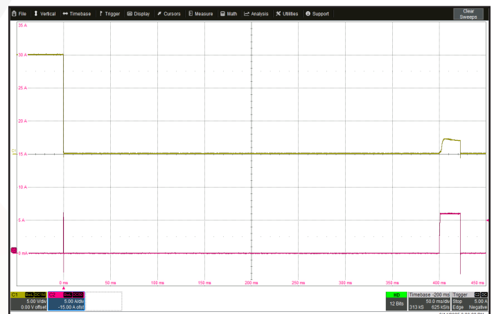
Figure 18: A short circuit across the output terminals. Ch 1: V_{out} (5 V/div). Ch 2: I_{out} (5 A/div). Time scale: 50.0 ms/div.
