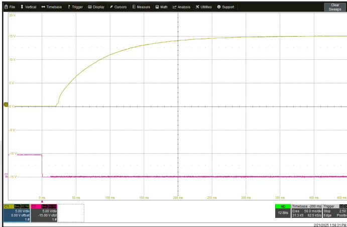
Figure 7: Turn-on transient at full load and zero output capacitance initiated by On/Off. Input voltage pre-applied. Ch 1: V_{out} (5 V/div). Ch 2: On/Off (5 V/div). Timescale: 50.0 ms/div.
