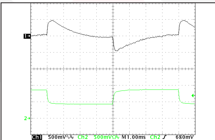
Figure 11: Output voltage response to step-change in load current 50%-100%-50% of Iout (max); dI/dt = 2 \text{ mA}/\mu\text{s} . No external load capacitance. Ch 1: Vout (500 mV/div). Ch 2: Iout (500 mA/div). (1 ms/div).
