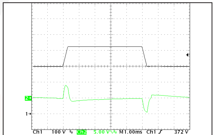
Figure 12: Output voltage response to step-change in input voltage (300 V - 425 V - 300 V); dV/dt = 400 \text{ V}/\text{ms} (rising). Ch 1: Vin (100 V/div). Ch 2: Vout (5 V/div). (1 ms/div).
