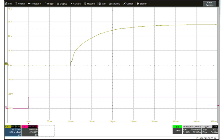
Figure 8: Turn-on transient at full load and zero output capacitance initiated by Vin. On/Off Pin previously low. Ch 1: Vout (10 V/div). Ch 2: Vin (500 V/div). Timescale: 50.0 ms/div.
