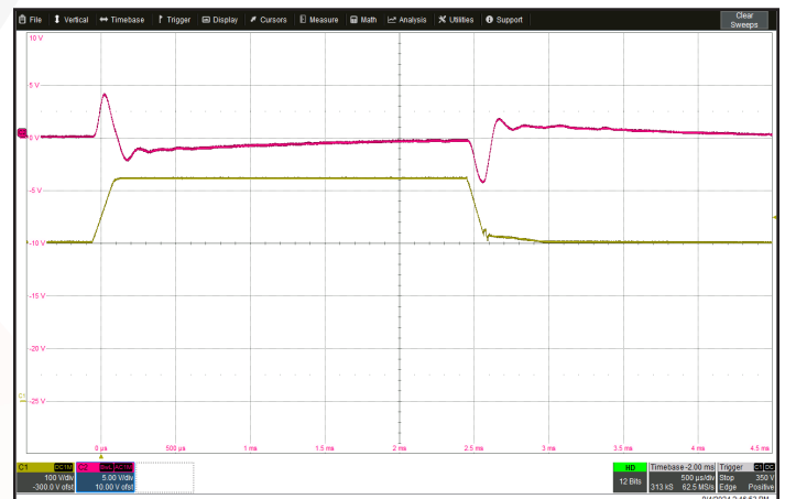
Figure 12: Output voltage response to step-change in input voltage (300 V - 425 V - 300 V) in 125 μs. Ch 1: Vin (100 V/div). Ch 2: Vout (5 V/div). Timescale: 500 μs/div.
