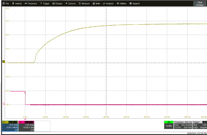
Figure 7: Turn-on transient at full load and zero output capacitance initiated by On/Off. Input voltage pre-applied. Ch 1: Vout (10 V/div). Ch 2: On/Off (5 V/div). Timescale: 50.0 ms/div.
